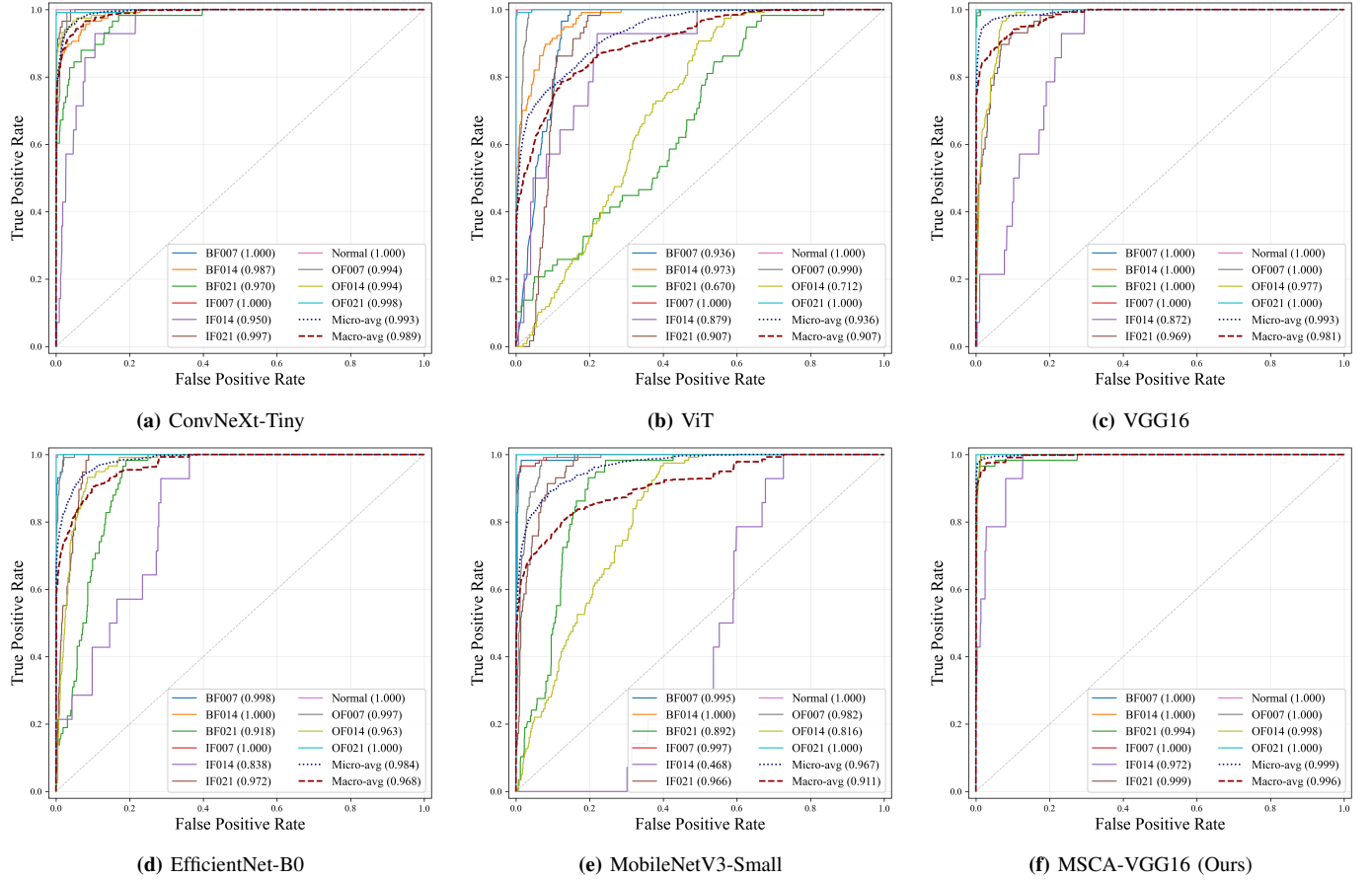
Fig. 10: ROC curves of different backbone networks on the CWRU 12k DE dataset. The proposed MSCA-VGG16 achieves higher AUC on most classes, indicating superior discriminative capability and robustness across classes.
