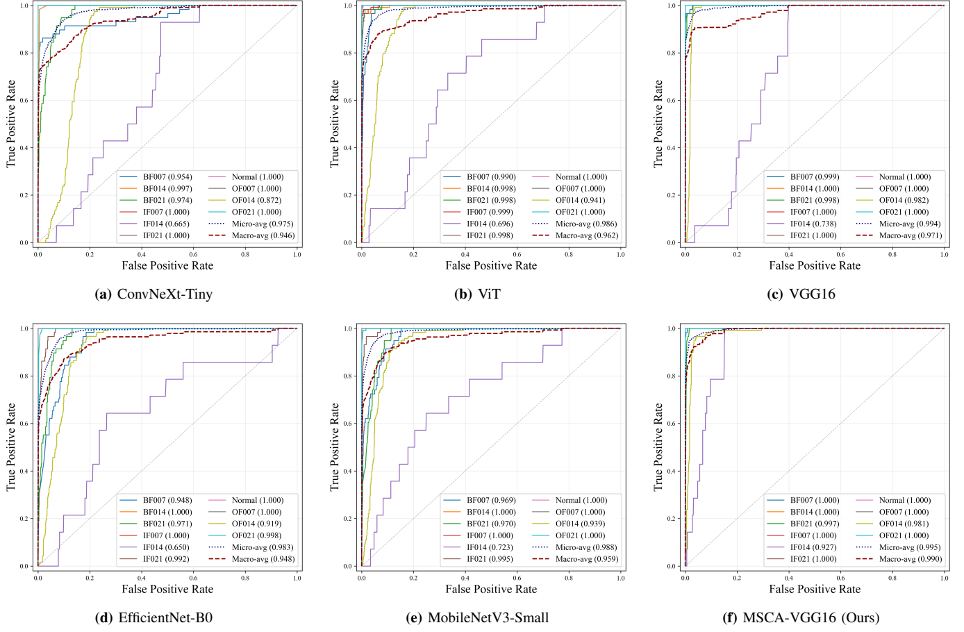
Fig. 10: ROC curves of different backbone networks on the CWRU 12k DE dataset. The proposed MSCA-VGG16 achieves the highest AUC, indicating superior discriminative capability and robustness across classes.
