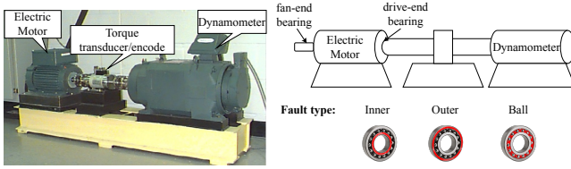
Fig. 6: CWRU bearing test stand. Vibration signals were collected from accelerometers at the drive-end and fan-end positions under four operating loads (0–3 hp).
