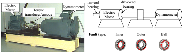
Figure 6: CWRU bearing test stand. Vibration signals were collected from accelerometers at the drive-end and fan-end positions under four operating loads (0–3 hp).
