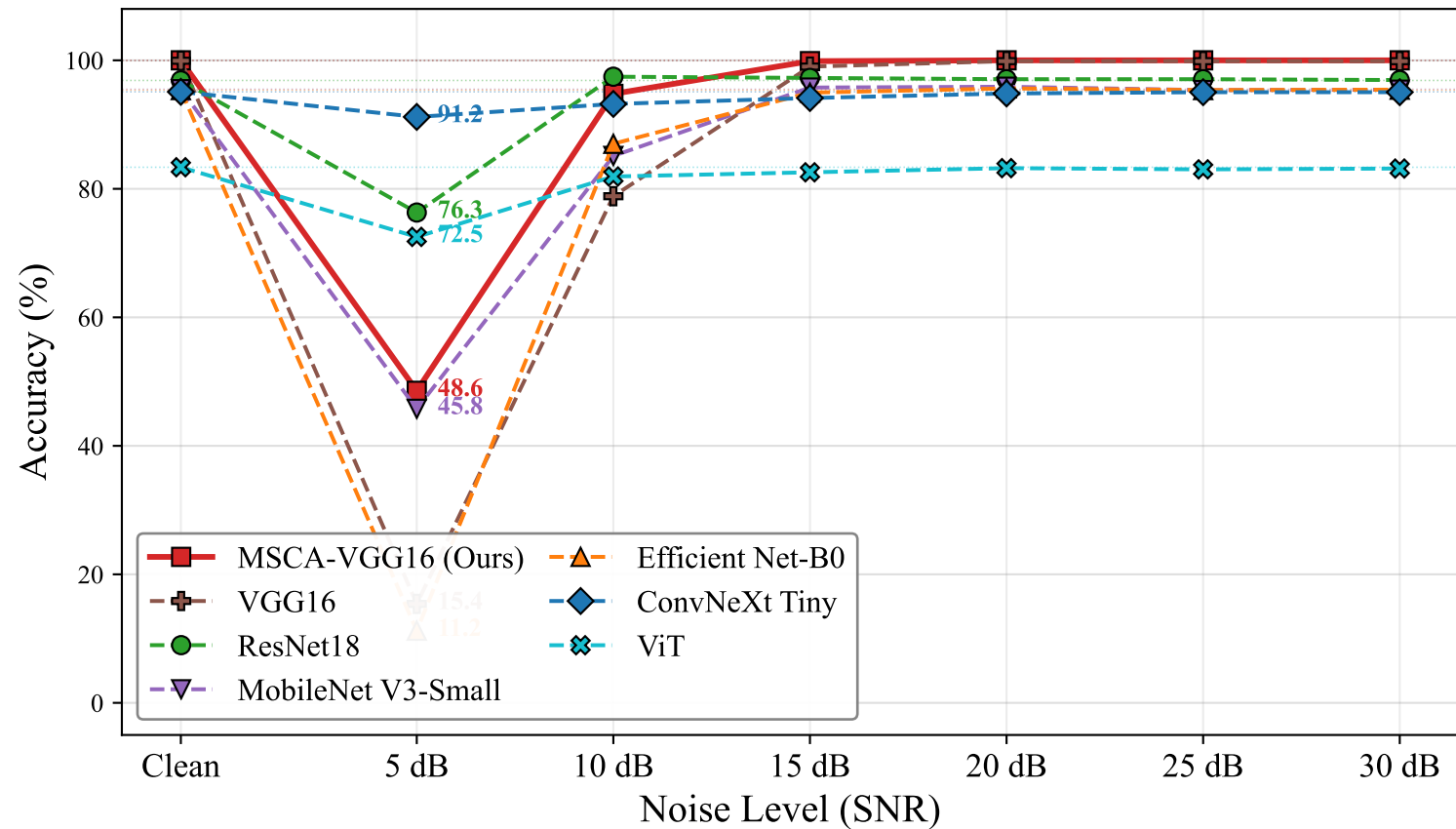
Noise Robustness Comparison — Accuracy vs SNR
