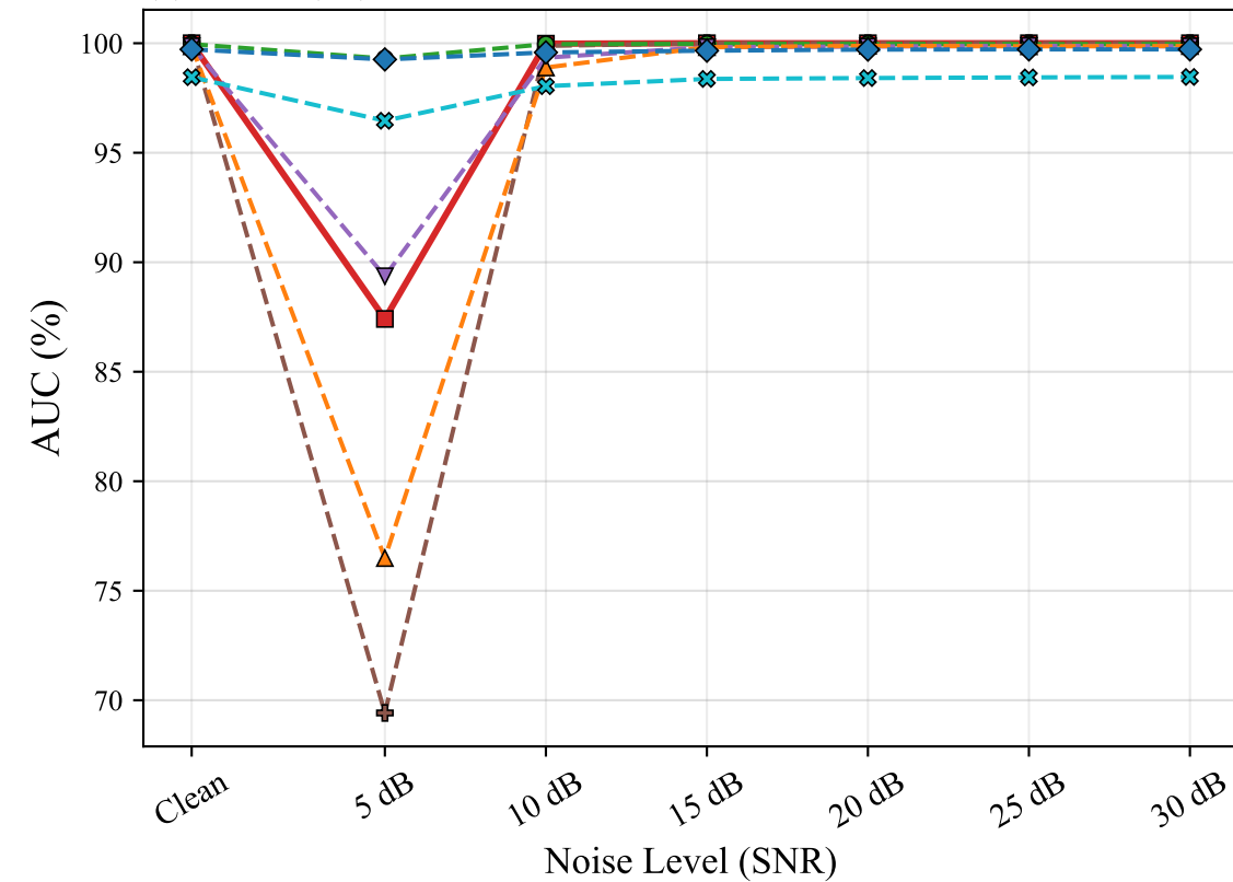
(c) AUC (%)
