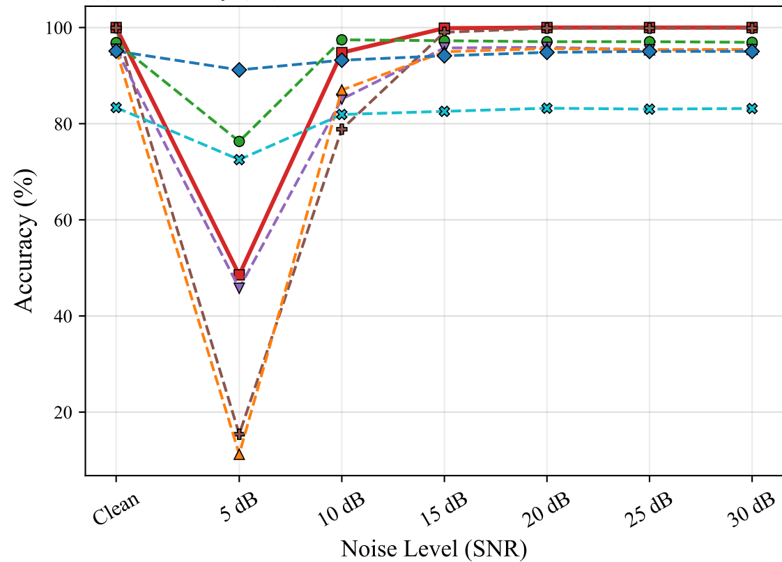
(a) Accuracy (%)
