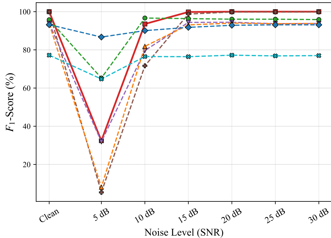
(b) F_1 -Score (%)
