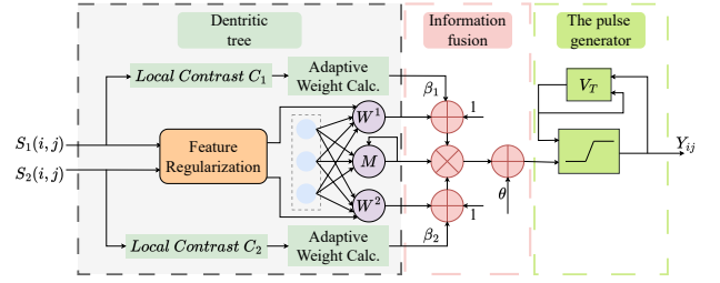
Fig. 3: Architecture of the proposed adaptive weighted dual-channel PCNN (AW-DPCNN) for multi-representation signal fusion.
