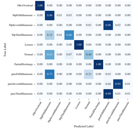
(b) AlexNet
