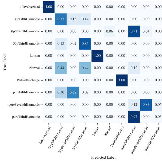
(c) ResNet18
