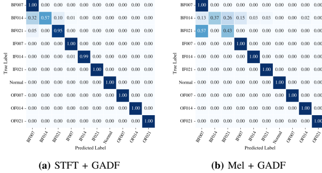
Fig. 7: Confusion matrices of the best-performing (STFT + GADF) and worst-performing (Mel + GADF) representation combinations. STFT + GADF exhibits substantially reduced inter-class confusion, particularly among fault severity levels.
