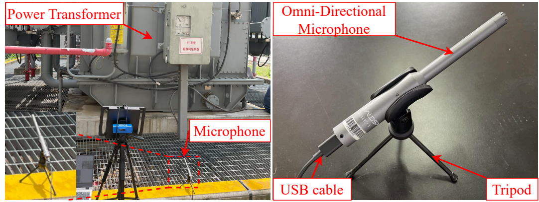
Figure 5: Experimental platform of acoustic signal acquisition.
