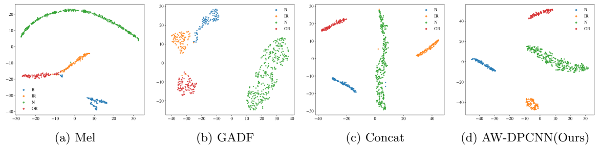
Figure 9: t-SNE visualization of feature distributions under different strategies. (a) A1: Mel representation. (b) A2: GADF representation. (c) A3: Mel+GADF with concatenation fusion. (d) A4: Mel+GADF with the proposed AW-DPCNN fusion, which produces more compact intra-class clusters and clearer inter-class boundaries.
