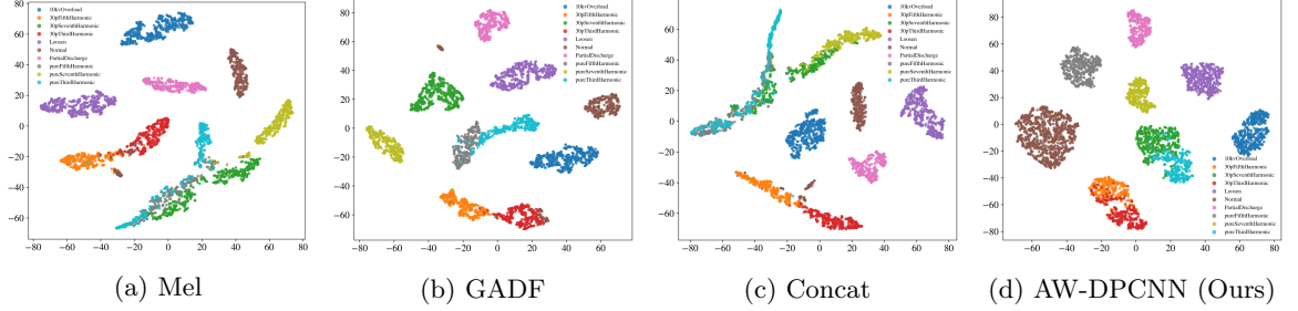
Figure 8: t-SNE visualization of feature distributions under different fusion mechanisms. (a) E1: Mel features. (b) E2: GADF features. (c) E3: Mel+GADF with concatenation fusion. (d) E4: Mel+GADF with the proposed AW-DPCNN fusion.
