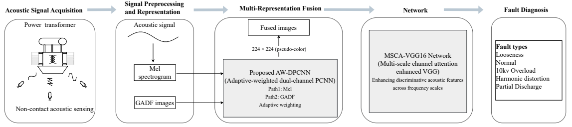
Figure 1: Overall framework of the proposed transformer acoustic diagnosis method. The acoustic signal is first converted into Mel spectrogram and GADF images. These heterogeneous representations are then adaptively fused through the proposed AW-DPCNN mechanism. Finally, the fused feature is fed into the MSCA-VGG16 network for fault diagnosis.
