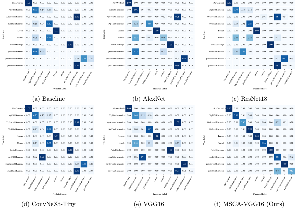
Figure 7: Confusion matrices of different network backbones trained using the AW-DPCNN fusion representations. The proposed MSCA-VGG16 achieves the most accurate classification performance with significantly reduced inter-class confusion.
