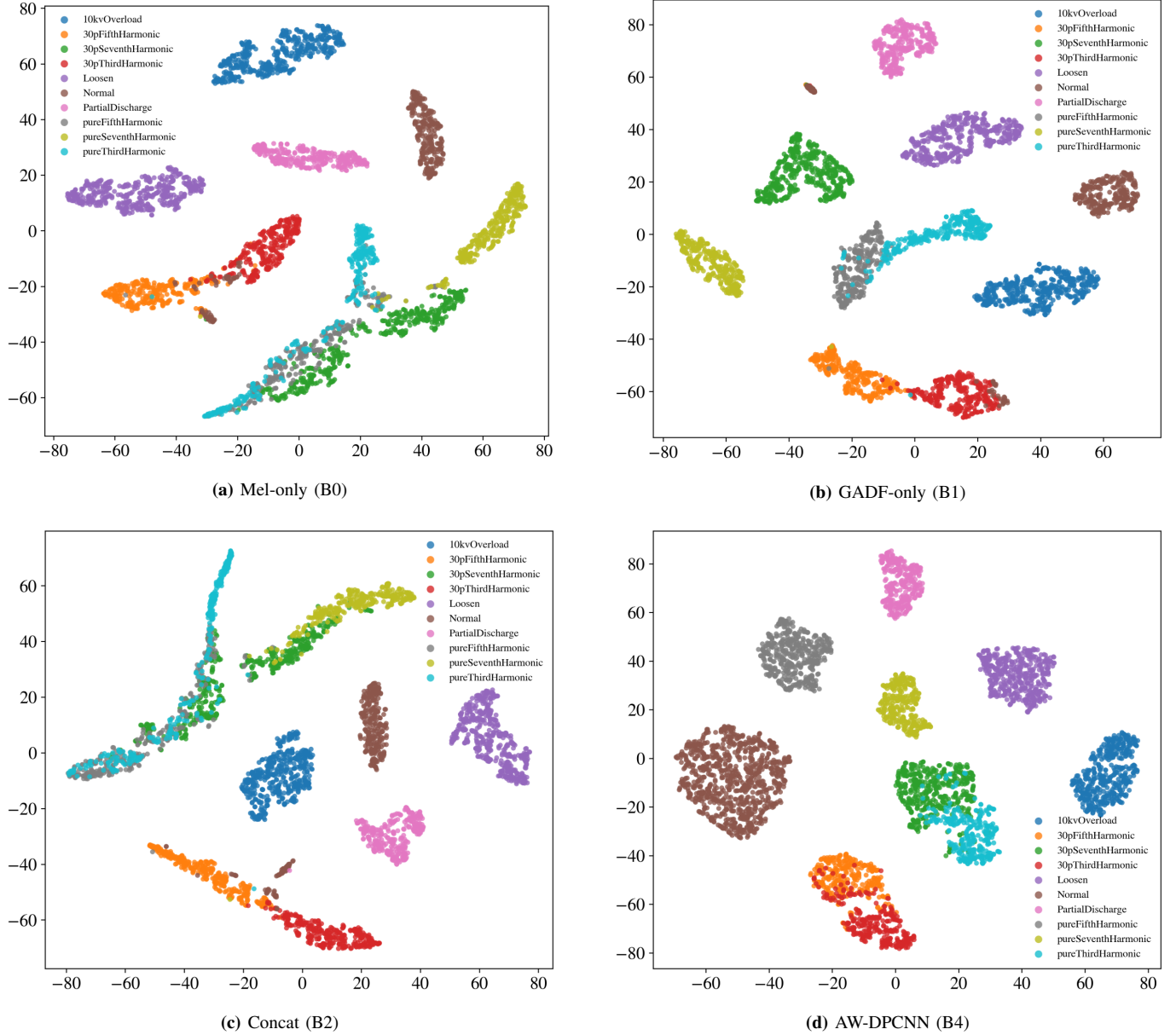
Fig. 9: t-SNE visualization of feature distributions under different fusion configurations. (a) B0: Mel-only. (b) B1: GADF-only. (c) B2: Mel+GADF concatenation. (d) B4: Full AW-DPCNN fusion, which yields the most compact intra-class clusters and the clearest inter-class separation.
