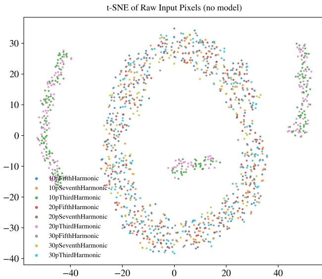
Fig. 10: t-SNE visualization of raw input pixels (PCA 50 → t-SNE) for the transformer acoustic dataset. Classes are severely overlapped, demonstrating that raw pixel features are not inherently separable.
