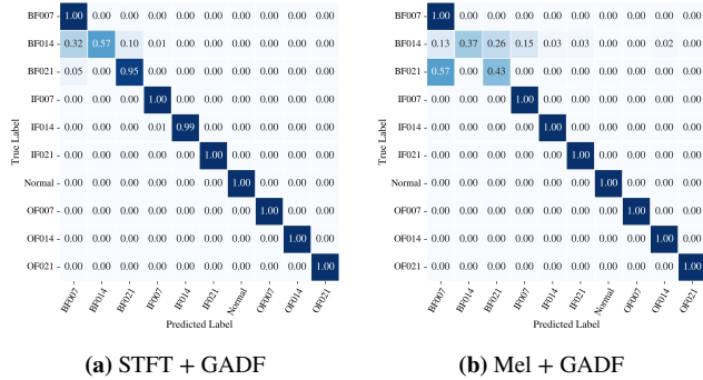
Figure 7: Confusion matrices of the best-performing (STFT + GADF) and worst-performing (Mel + GADF) representation combinations. STFT + GADF exhibits substantially reduced inter-class confusion, particularly among fault severity levels.
