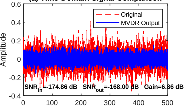
(a) Time-Domain Signal Comparison
