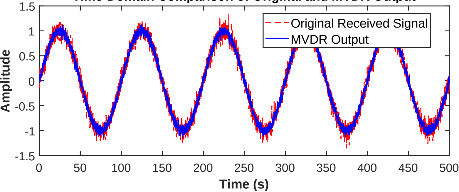
Time-Domain Comparison of Original and MVDR Output
