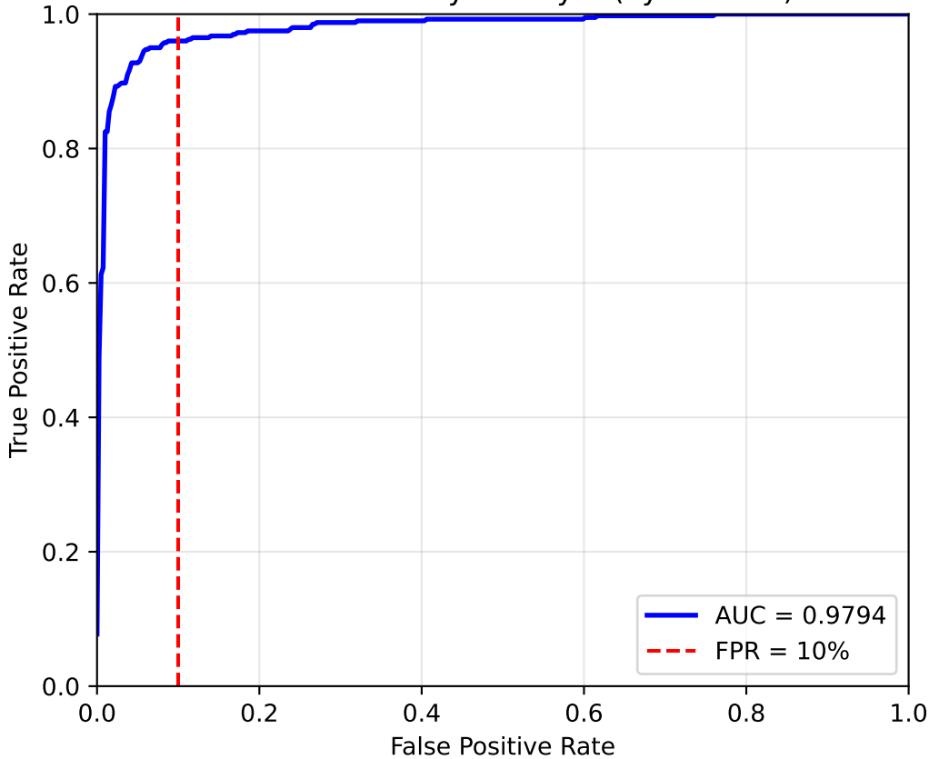
ROC Curve — ToyConveyor (PyTorch AE)
