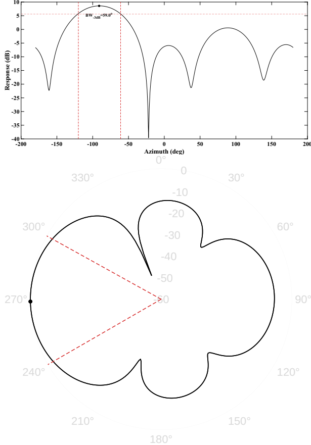
Fig. 12: Beam pattern of the MVDR beamformer at 2 kHz. The main lobe is directed towards the target signal, while deep nulls are observed in the direction of the interference, indicating effective spatial filtering.
