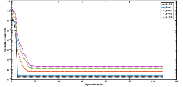
Fig. 6: Covariance eigenspectra of the composite received signal as functions of wall reflection coefficient. Eigenvalues are regularized with diagonal loading. The curves demonstrate the progressive deterioration of signal-to-noise eigenvalue separation with increasing room reverberation.
