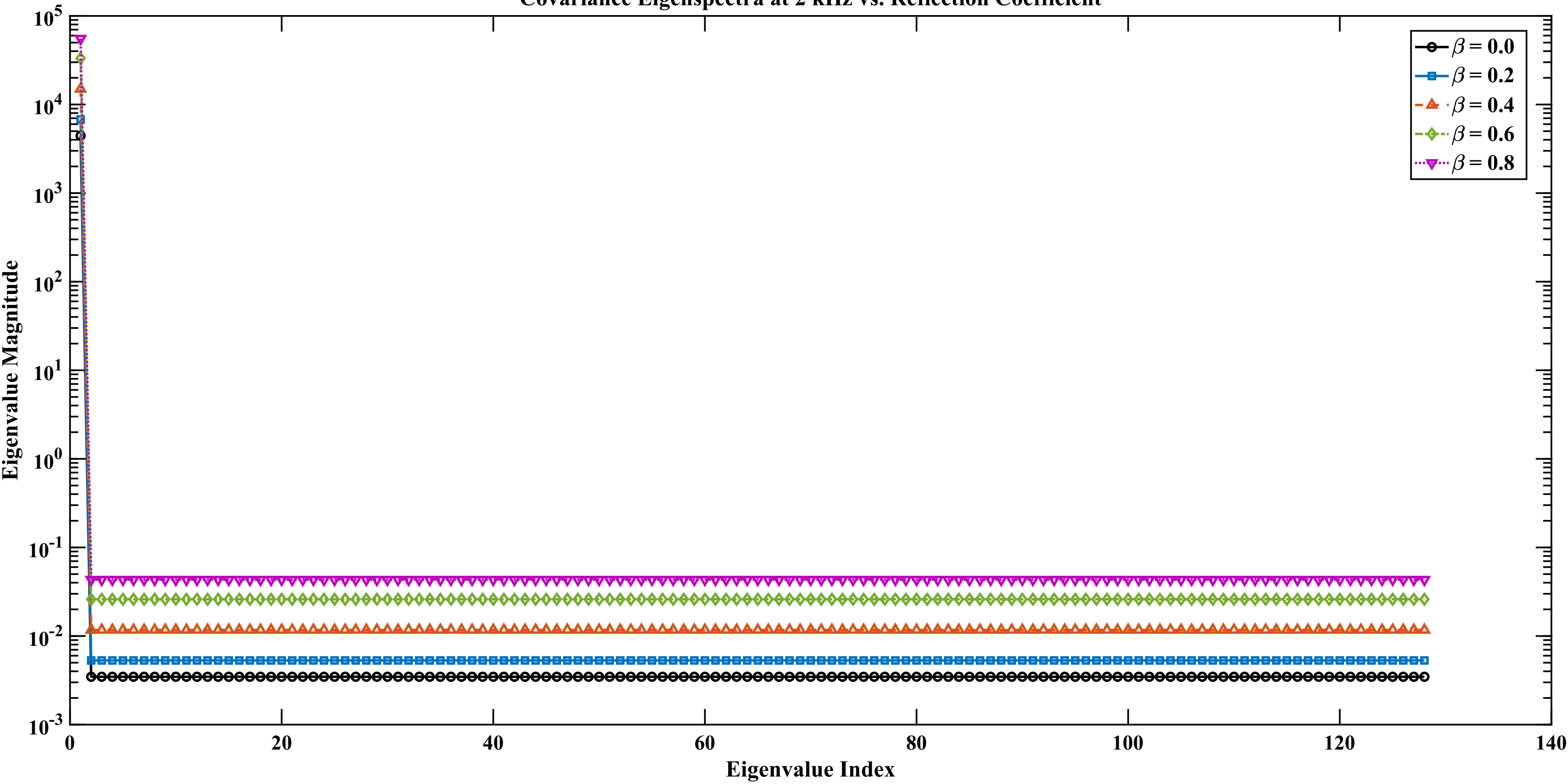
Covariance Eigenspectra at 2kHz vs. Reflection Coefficient
