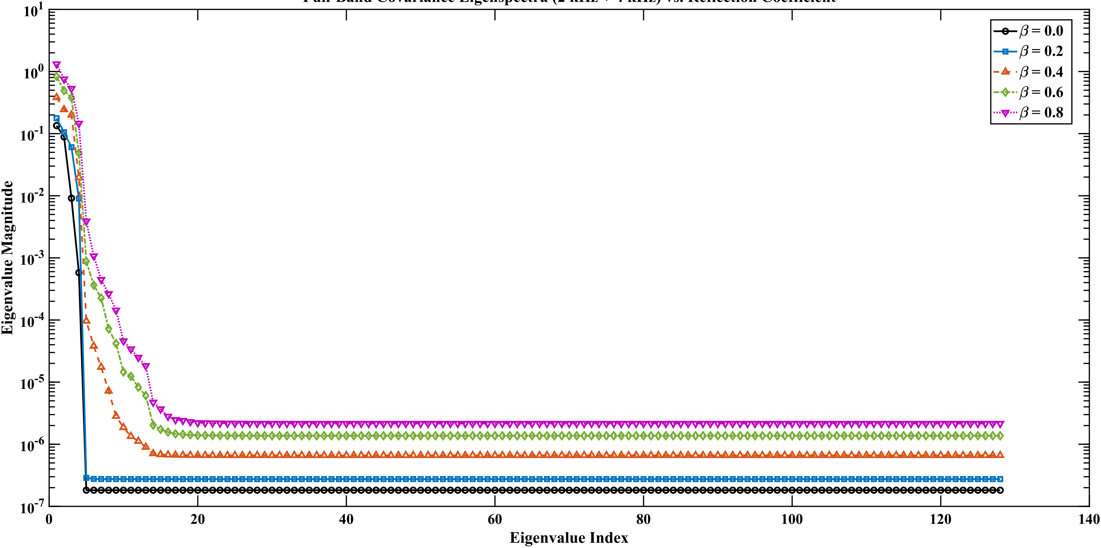
Full-Band Covariance Eigenspectra (2 kHz + 4 kHz) vs. Reflection Coefficient
