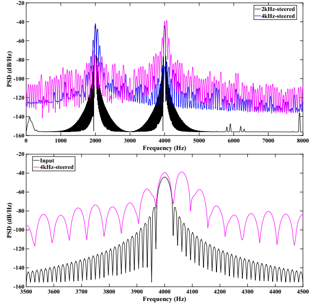
Fig. 3: Power Spectral Density (PSD) of the target and interference signals after RIR convolution. We steered the target to the 2kHz and 4kHz signal, respectively.
