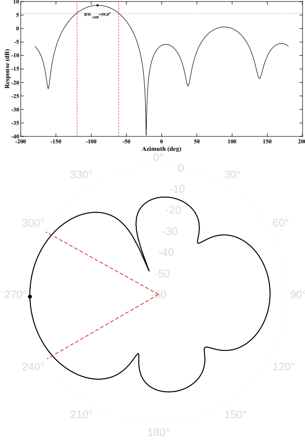
Fig. 12: Beampattern of the MVDR beamformer at 2 kHz. The main lobe is directed towards the target signal, while deep nulls are observed in the direction of the interference, indicating effective spatial filtering.
