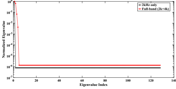
Fig. 4: Eigenvalue spectrum of the covariance matrix at the 2 kHz frequency bin. The significant gap between the largest eigenvalue and the others indicates a strong spatial structure, favorable for MVDR beamforming performance.
