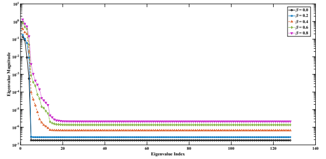
Fig. 6: Covariance eigenspectra of the composite received signal as functions of wall reflection coefficient \beta . Eigenvalues are regularized with diagonal loading. The curves demonstrate the progressive deterioration of signal-to-noise eigenvalue separation with increasing room reverberation.
