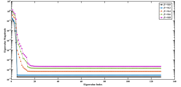
Fig. 6: Covariance eigenspectra of the composite received signal as functions of wall reflection coefficient \beta . Eigenvalues are regularized with diagonal loading. The curves demonstrate the progressive deterioration of signal-to-noise eigenvalue separation with increasing room reverberation.
