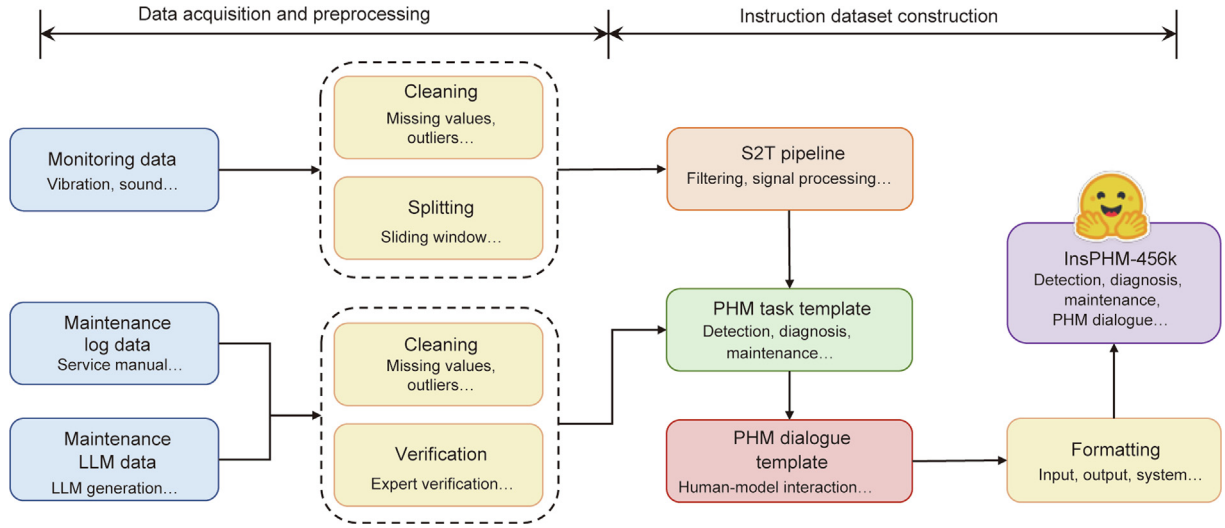
Fig. 5. The instruction dataset construction method of InstPHM-456k.
