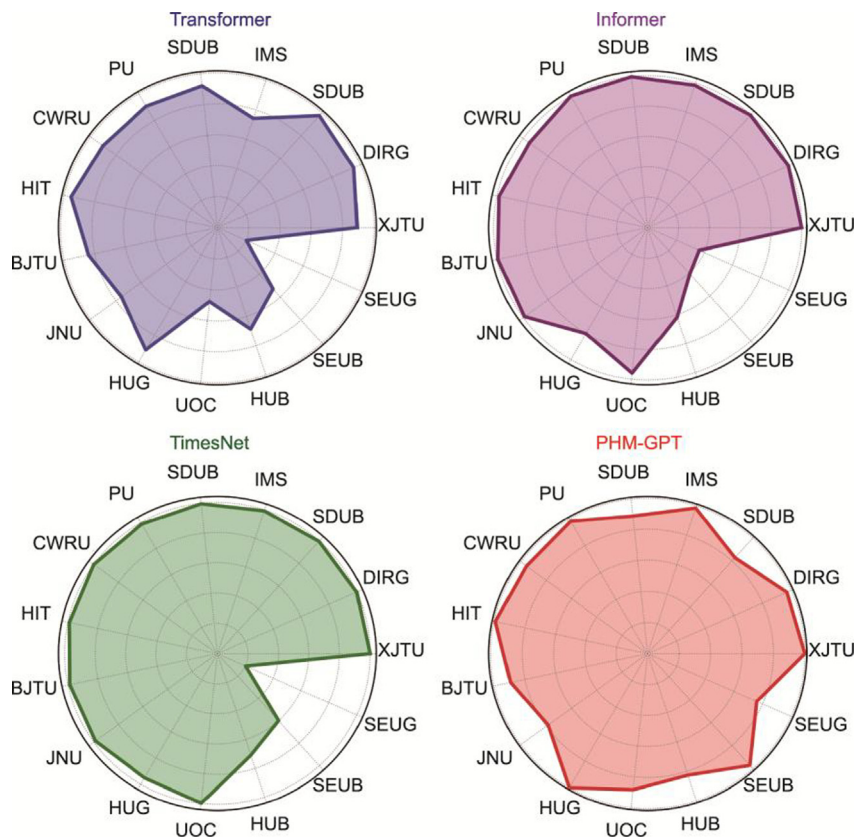
Fig. 10. Diagnostic accuracy comparison among typical models in the fault diagnosis task.
