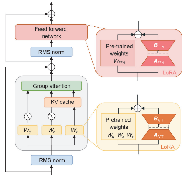
Fig. 6. One of the decoder blocks in our architecture design.
