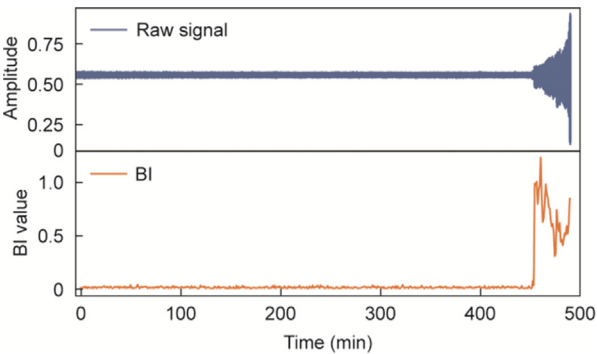
Fig. 15. Visualization of the BI values produced for XJTU-SY bearing 2–1.
