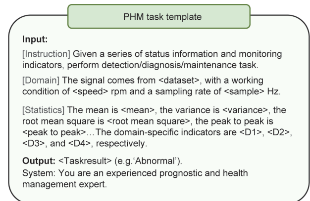
Fig. 2. The instruction template for PHM task. rpm: revolutions per minute.
