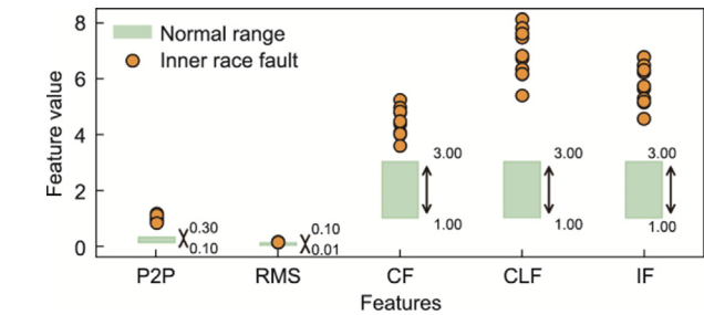
Fig. 14. Visualization of the thresholds produced in the threshold-setting case study.
