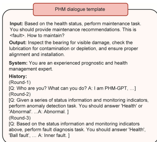
Fig. 3. The instruction template for PHM dialog.
