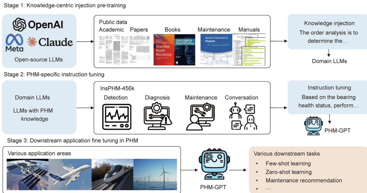
Fig. 7. Framework for generalizing the PHM-GPT from pretraining to downstream tasks.
