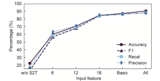
Fig. 11. Impact of the number of features contained in the S2T pipeline on the performance of the model.
