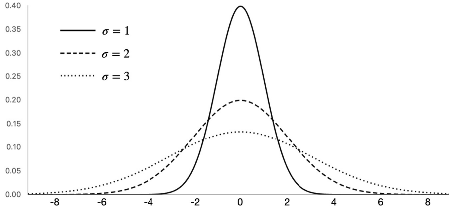
Figure 8.2: Gaussian distributions with centers c = 0 and standard deviations \sigma = 1, 2, 3 .
