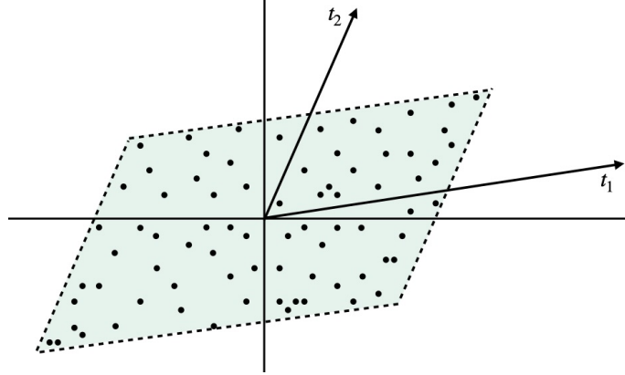
Figure 8.1: Signature points s in the parallelepiped P_{1/2}(T) = \{a_1 t_1 + a_2 t_2 : -\frac{1}{2} \leq a_i \leq \frac{1}{2}\} .
