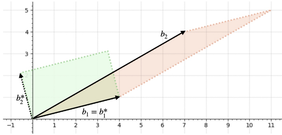
Figure 9.2: The fundamental parallelepipeds spanned by the lattice vectors b_1 = (4, 1) and b_2 = (7, 4) (shaded red), and by the Gram-Schmidt vectors b_1^* = (4, 1) and b_2^* = (-9/17, 36/17) (shaded green); both have area 9.
