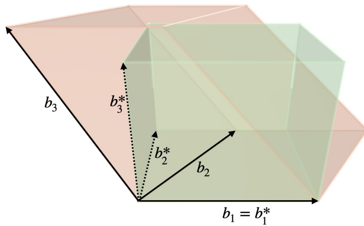
Figure 9.3: The fundamental parallelepipeds spanned by the lattice vectors b_1 = (6, 1, 0) , b_2 = (3, 5, 0) and b_3 = (-6, 3, 5) (shaded red), and by the Gram-Schmidt vectors b_1^* = (6, 1, 0) , b_2^* = (-27/37, 162/37, 0) and b_3^* = (0, 0, 5) (shaded green); both have volume 135.
