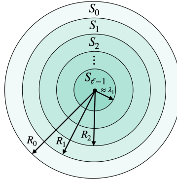
Figure 10.1: The sieving method.
