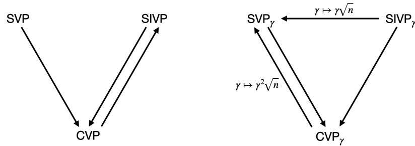
Figure 2.5: The known relationships between SVP, SIVP, CVP, and their approximate versions. An arrow A \rightarrow B indicates that A polynomial-time reduces to B . Any loss in the approximation factor incurred by the reduction is shown next to the arrow.
