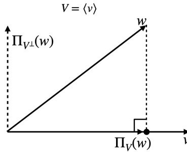
Figure 9.1: The projections of w onto V and V^\perp .
