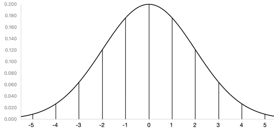
Figure 8.4: The one-dimensional discrete Gaussian distribution D_{\mathbb{Z},5} .
