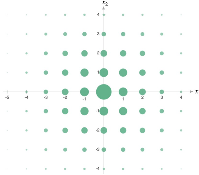
Figure 8.5: The two-dimensional discrete Gaussian distribution D_{\mathbb{Z}^2, 3} . Each circle is centered at a lattice point x = (x_1, x_2) \in \mathbb{Z}^2 , with radius proportional to \rho_3(x) .
