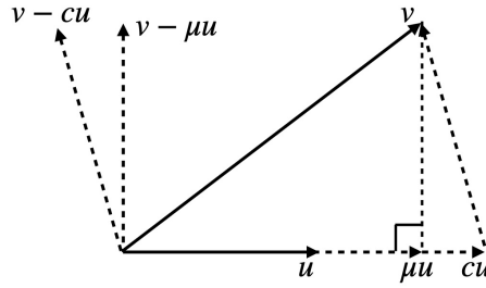
Figure 9.4: An iteration of Gauss's algorithm.
