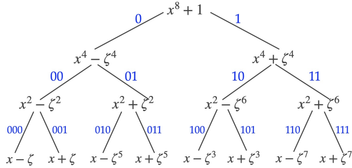
Figure 12.1: The NTT computation tree ( n = 8 ).
