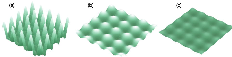
Figure 8.6: The function f(x) = \sum_{c \in L} D_{s,c}(x) for increasing widths s .
