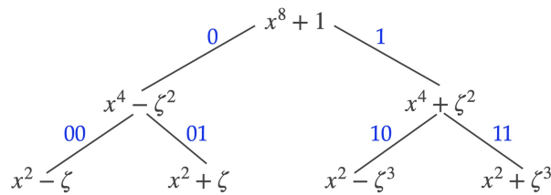
Figure 12.5: The \text{NTT}_2 computation tree ( n = 8 ).
