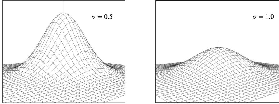
Figure 8.3: Two-dimensional Gaussian distributions with standard deviations \sigma = 0.5 , 1.0 .
