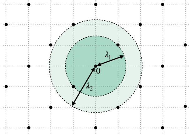
Figure 2.2: Successive minima.
