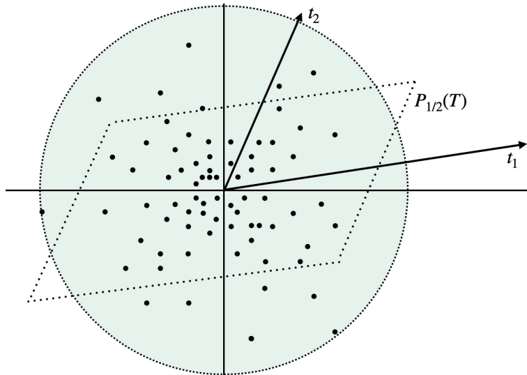
Figure 8.7: Signature points s in the GPV signature scheme; cf. Figure 8.1.
