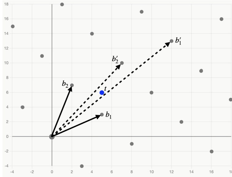
Figure 2.4: Finding a close lattice vector using rounding (cf. Example 2.24).
