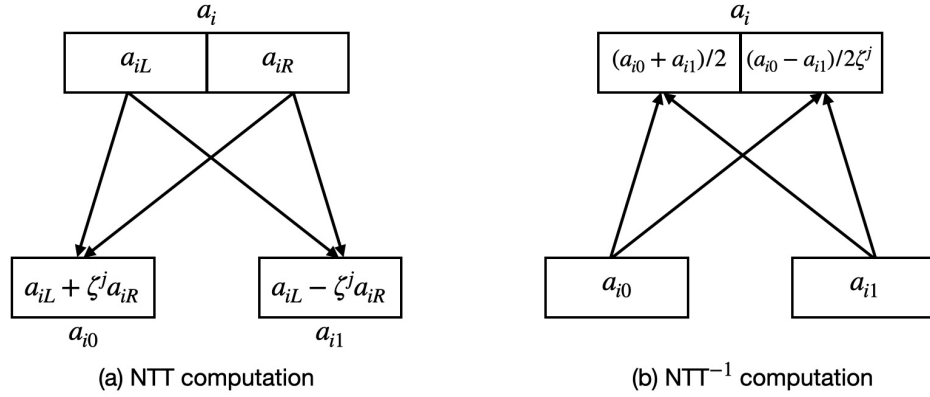
Figure 12.3: The “butterfly” formulas for computing NTT and \text{NTT}^{-1} .
