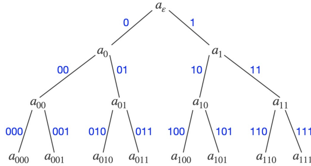
Figure 12.2: The NTT tree for n = 8 .
