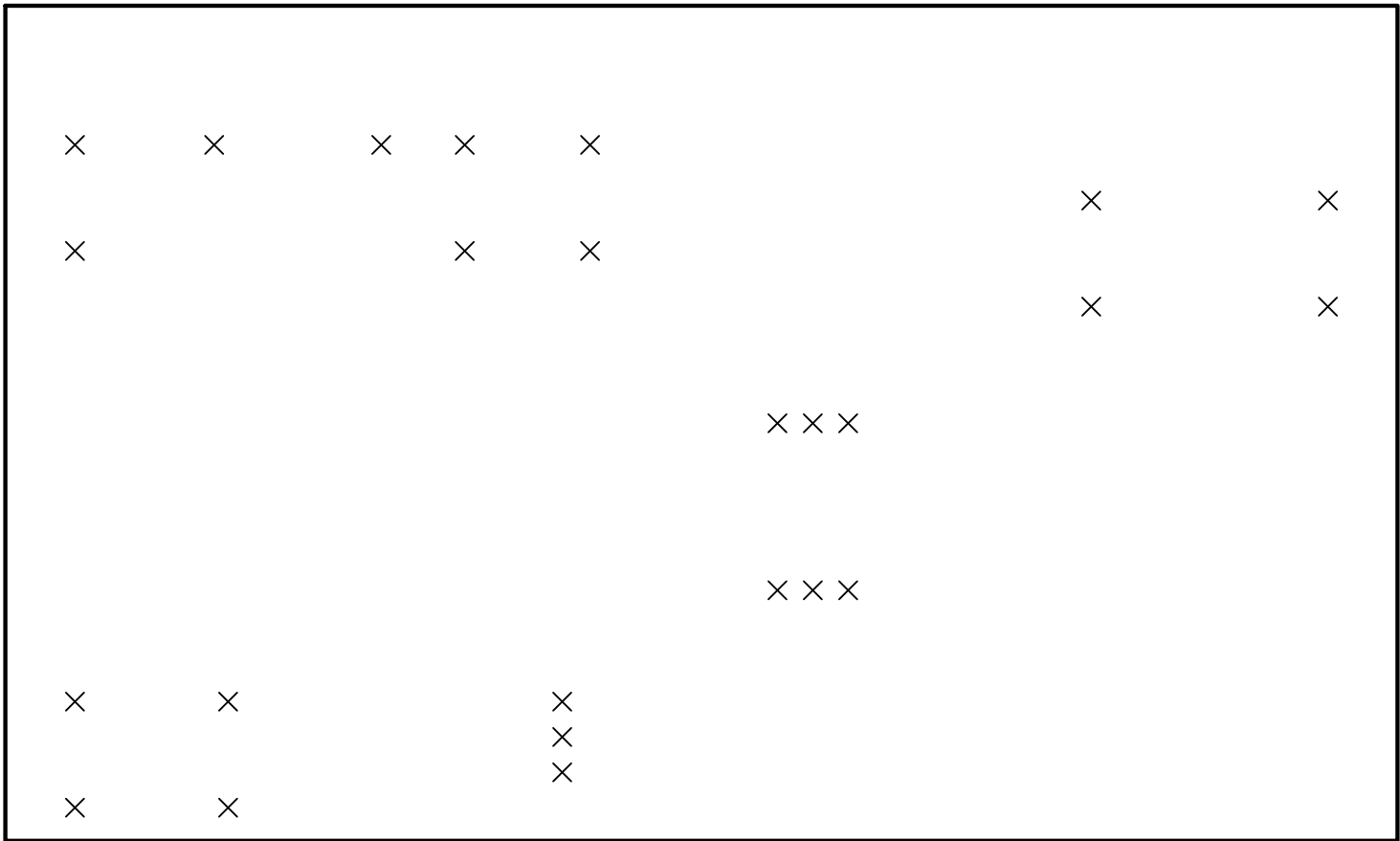
Drill Map: X 1.300mm / 0.0512" (25 holes)
