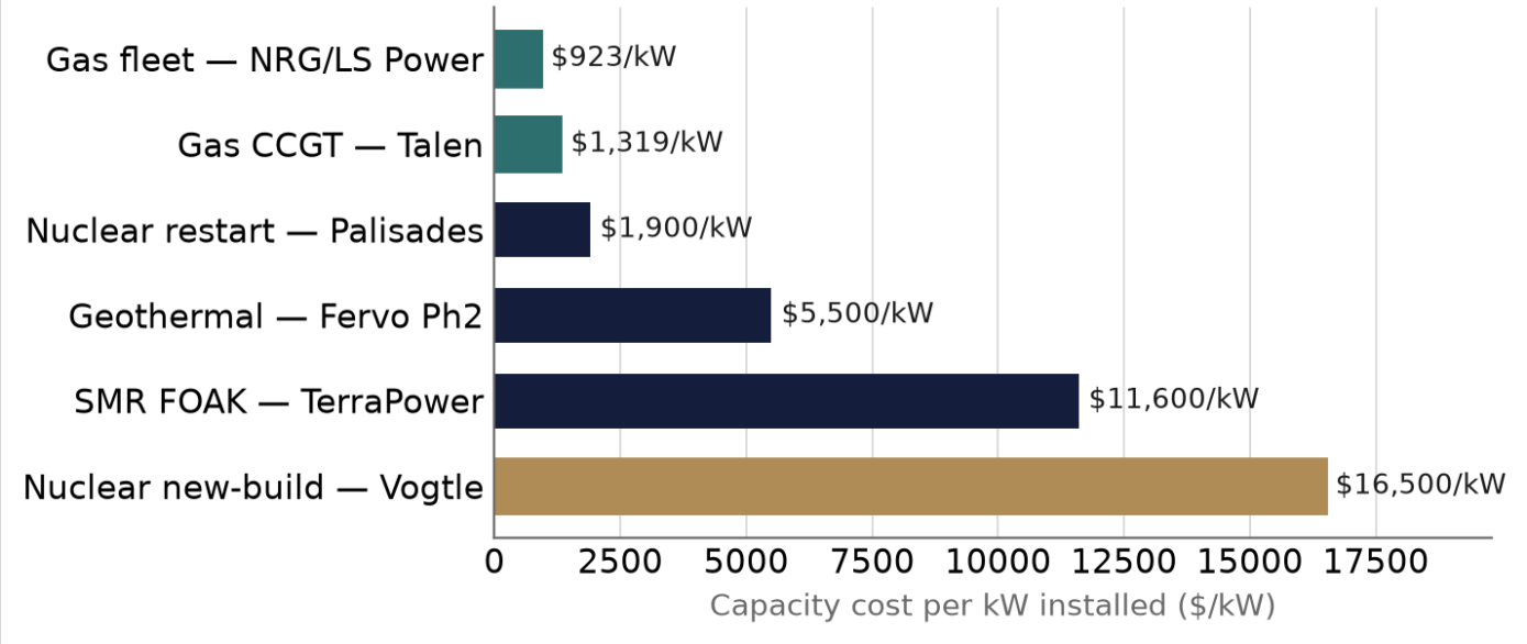
Fig. 3 — What one kW of firm capacity costs across the stack: operating gas fleets and nuclear restarts are an order of magnitude cheaper per kW than greenfield nuclear (Vogtle). Sources: Sections B, D, E.
