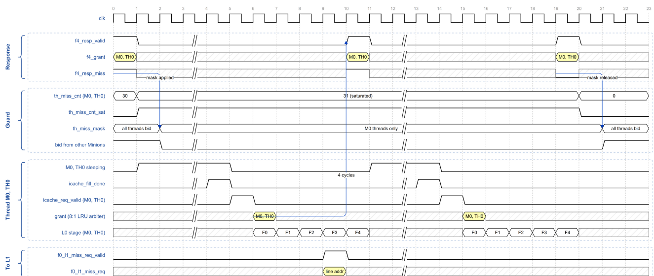
Figure 32. Counter saturation, bid mask and release
