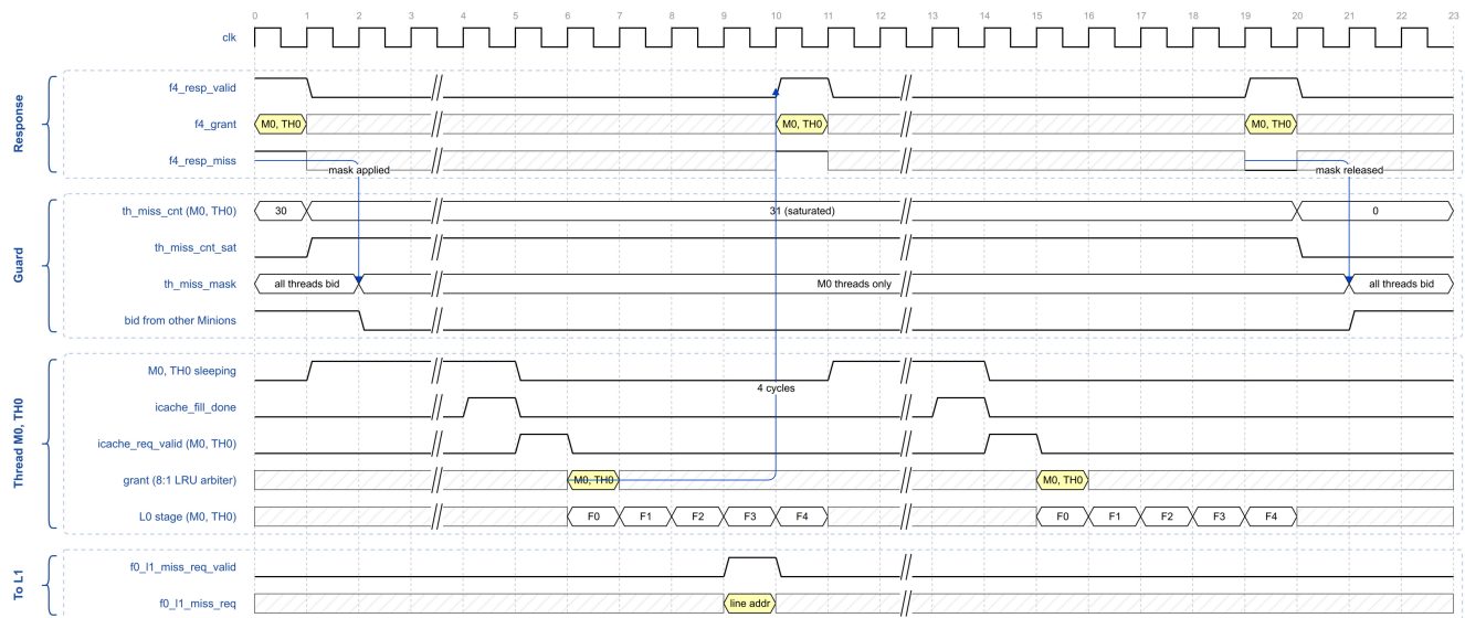
Figure 28. Miss-count guard: saturation, bid mask and release
