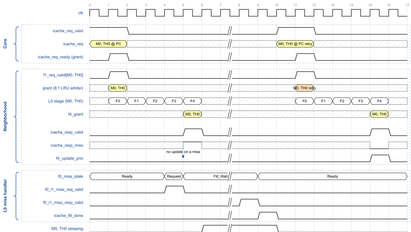
Figure 25. Miss, sleep, fill done and retry
