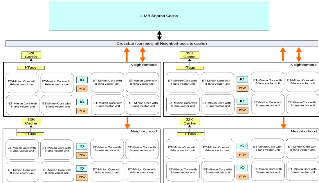
Figure 4. Minion Shire with four Neighborhoods and the 4 MB Shire Cache
