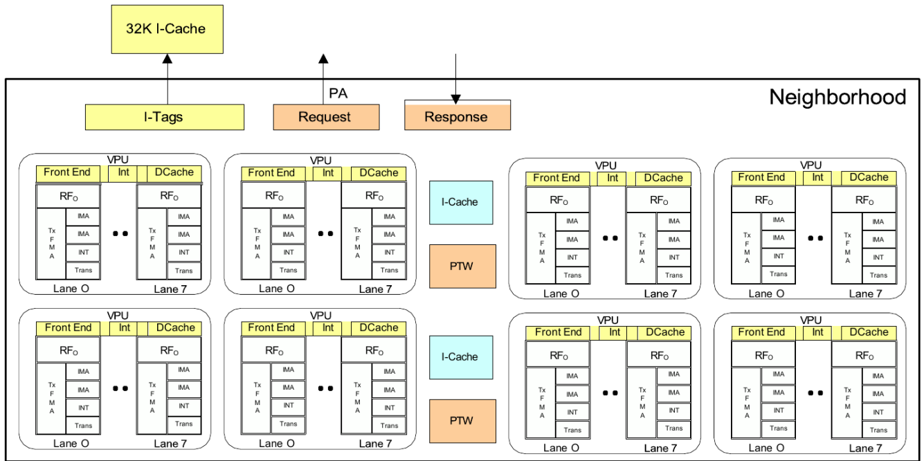
Figure 3. Neighborhood. Each group of four cores shares one L0 micro-cache (labeled "I-Cache") and one PTW. All eight cores share the 32 KB L1 instruction cache.
