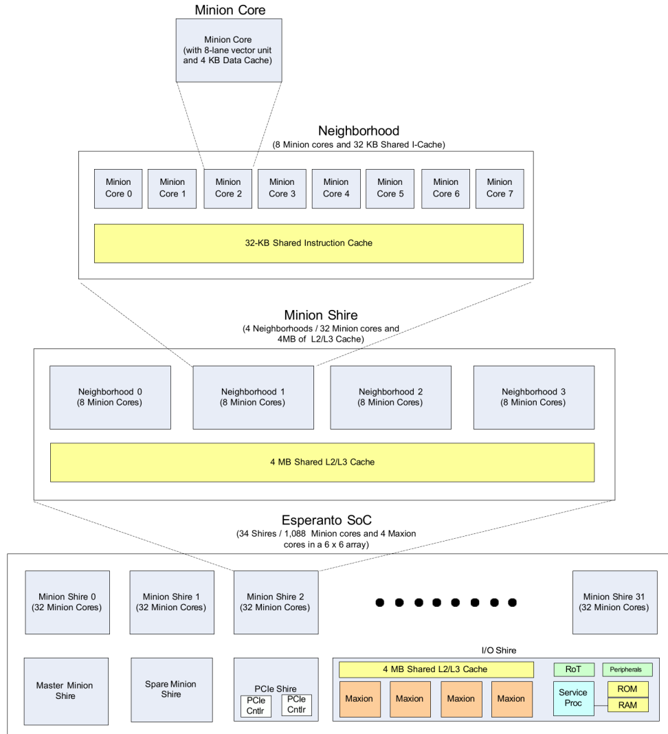
Figure 1. ET-Minion hierarchy, from core to device
