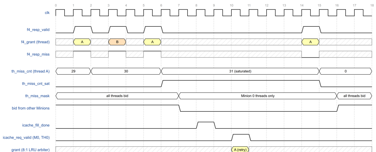
Figure 32. Counter saturation, bid mask and release
