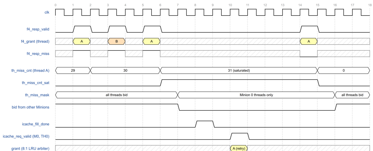
Figure 28. Miss-count guard: saturation, bid mask and release
