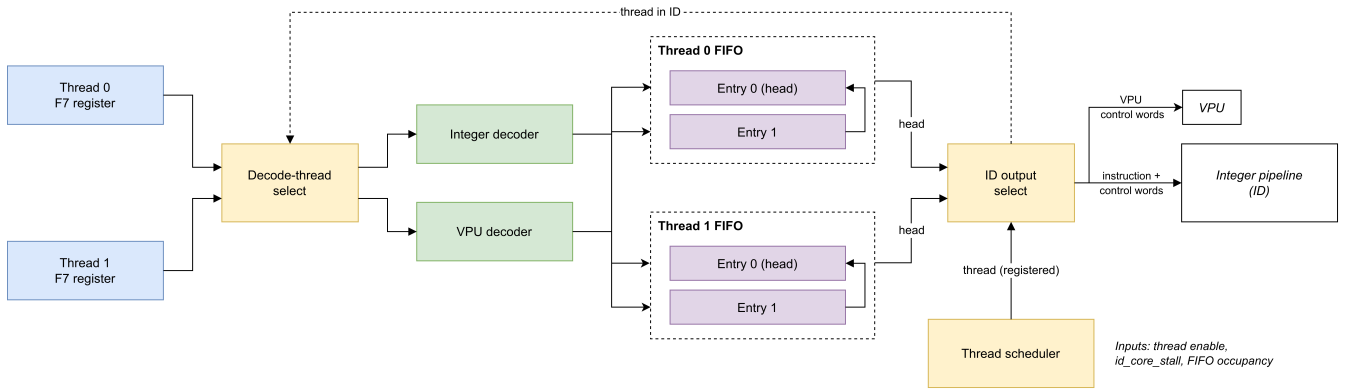
Figure 20. Decoders, instruction FIFOs and thread scheduler
