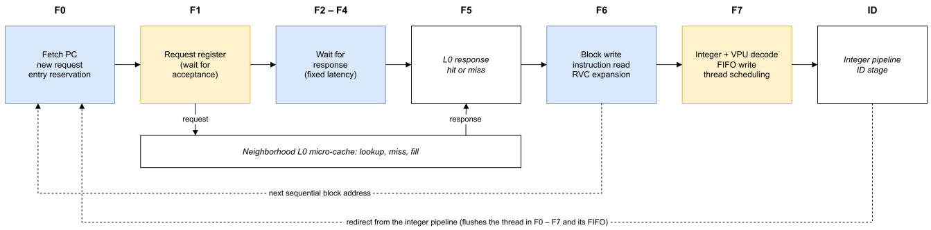
Figure 10. Front End pipeline
