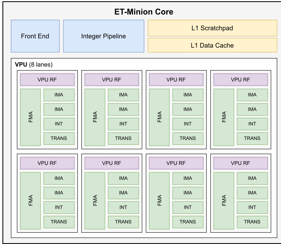
Figure 2. ET-Minion core
