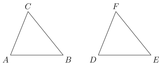
Figure 1: SAS Congruence
