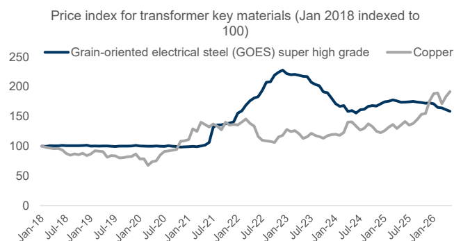
Exhibit 8: Key raw materials for transformer, GOES, saw prices inch down
