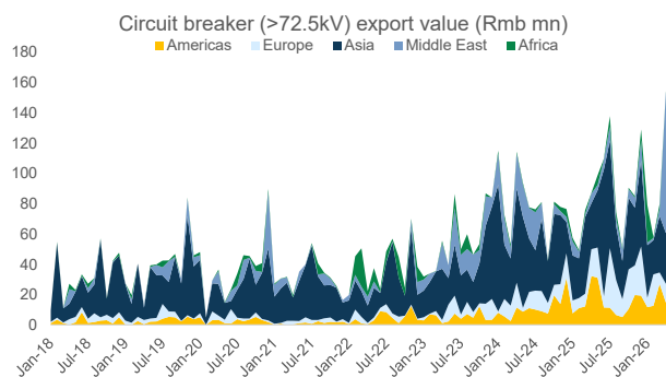
Exhibit 12: China circuit breaker (>72.5kV) export value was -7% yoy in June (vs -16% yoy in May)
