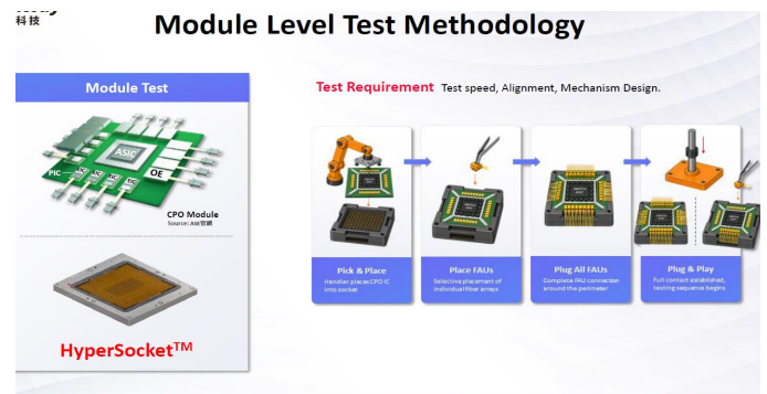
Fig. 14: WinWay proposes HyperSocket for CPO module test
