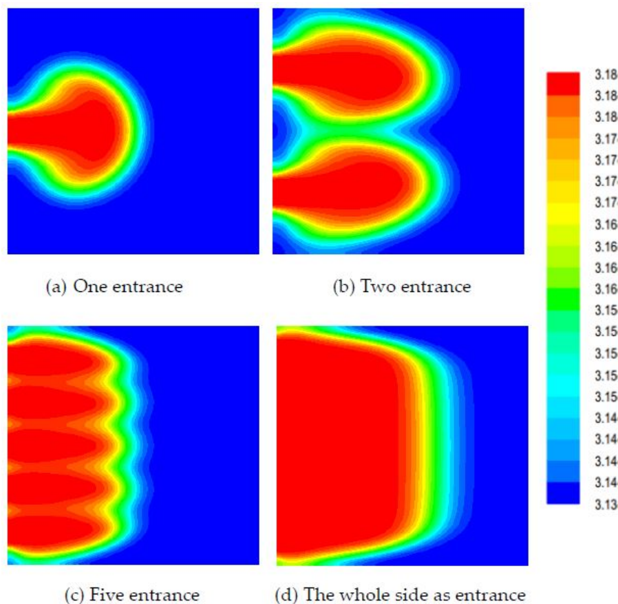
Figure 6: The simulation results of different ways of arranging entrances
