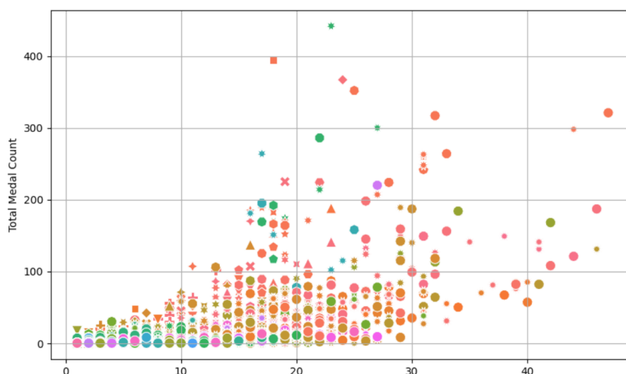
Figure 17: The relationship between the number of medals and the number of sports events participated in
