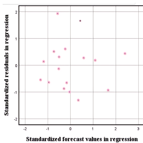
Figure 8: Residual plot
