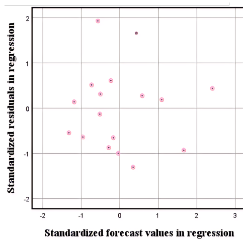
Figure 6: Residual plot
