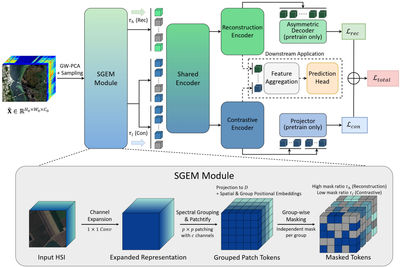
Fig. 1. Overall architecture of the proposed MSG framework. The model performs coordinated dual-objective pretraining, comprising a reconstruction objective with a high masking ratio and a contrastive objective with a low masking ratio. The SGEM module converts hyperspectral samples into spectral-grouped patch tokens, which are fed into the shared encoder and branch-specific heads. The bottom illustrates the detailed workflow of the SGEM module.
