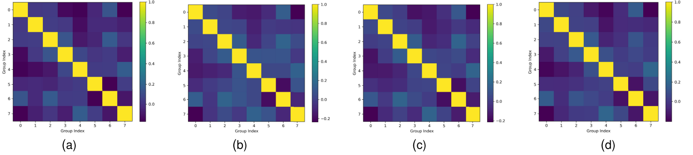
Fig. 3. Visualization of group-wise cosine similarity matrices on four downstream datasets. Each matrix is computed from a randomly sampled patch using the pretrained SGEM. Brighter diagonal entries and low off-diagonal responses indicate strong intragroup coherence and weak intergroup correlation. (a) Berlin. (b) Salinas. (c) WHU-Hi-LongKou. (d) Houston2013.
