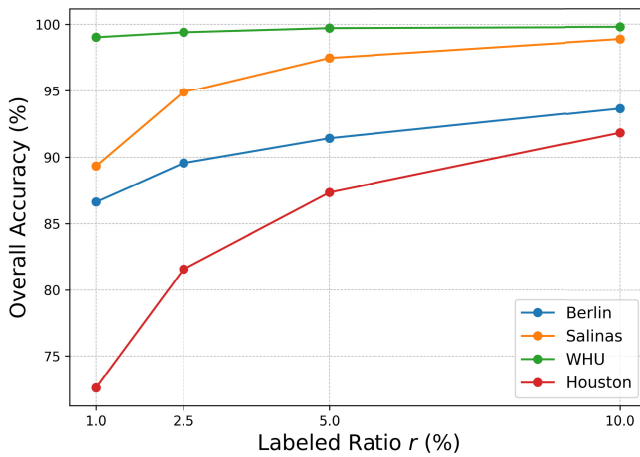
Fig. 5. OA versus labeled ratio r under FT.
