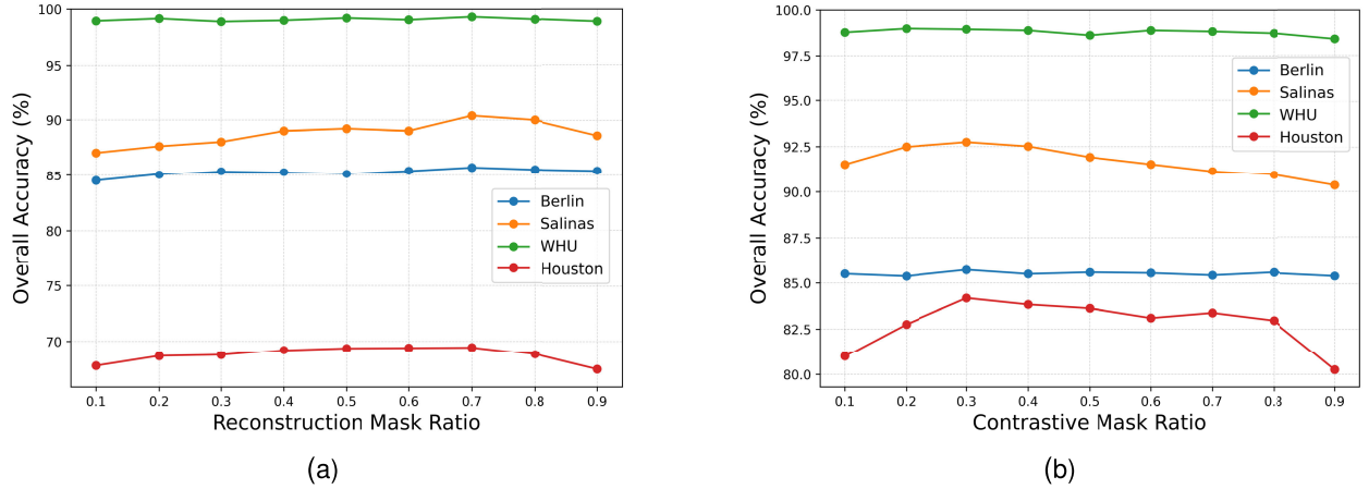
Fig. 4. Sensitivity to mask ratios for (a) reconstruction branch and (b) contrastive branch. Results are obtained under single-branch settings following Groups 3 and 4 of the component ablation in Table X.
