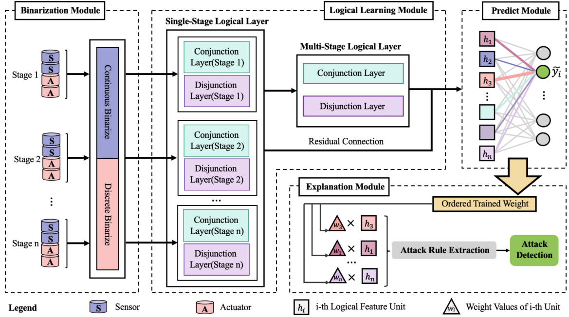
Fig. 1. Overview of the structure of ALRL.
