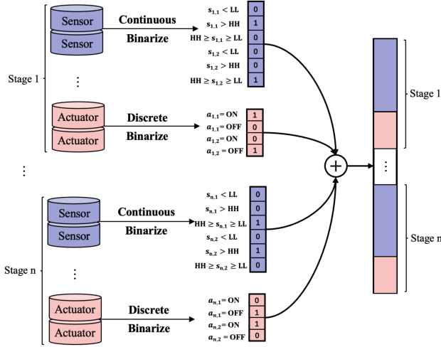
Fig. 2. Structure of the binarization module.
