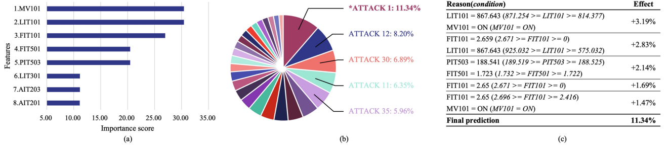
Fig. 5. Explaining a sample of Attack 1 on the SWaT dataset. (a) A summary plot of top important features in predicting attack class 1. (b) A pie chart shows the predict probability based on the top 5 important features, label marked with asterisks denote the decision outcomes. (c) A contribution table illustrates how the important features of the sample effect the prediction of attack class 1.
