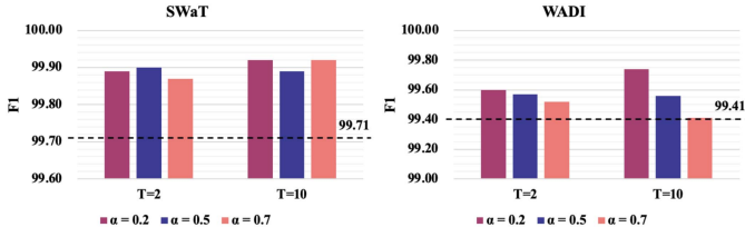
Fig. 4. Attack classification performances using different values of \alpha and T . The black dashed line shows the performance when \alpha = 0 .
