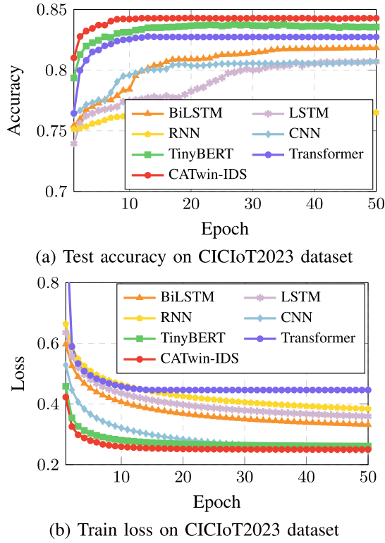
Fig. 6. Comparison of EVN performance indicators on CICIOT2023 dataset.
