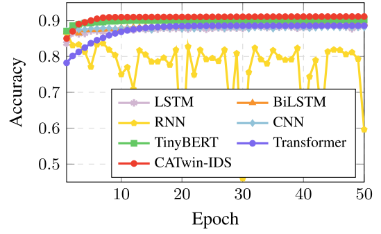
(a) Test accuracy on CICIDS2018 dataset
