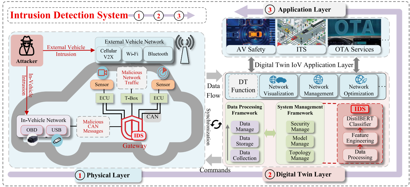
Fig. 2. Application scenario diagram of digital twin intrusion detection system for IoV.
