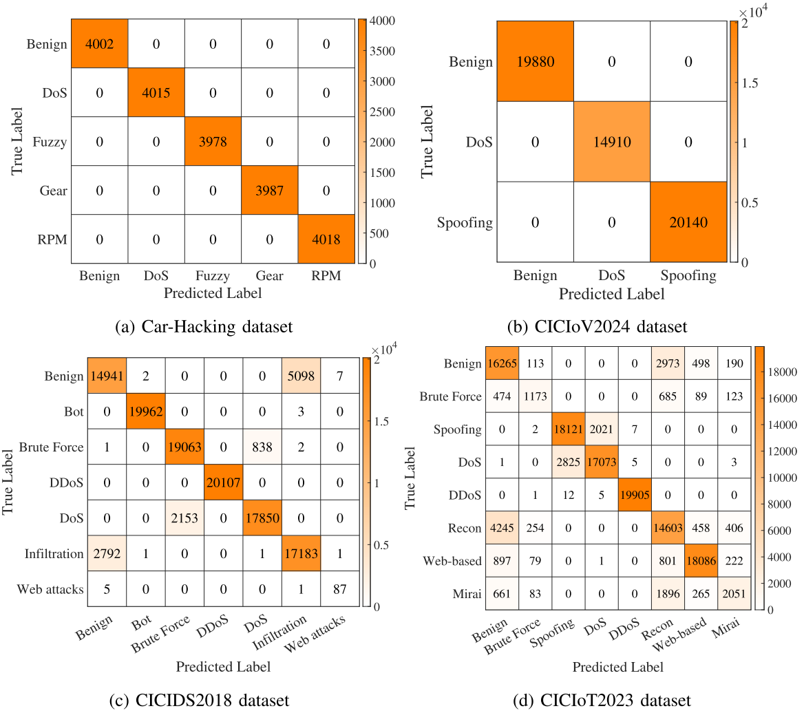
Fig. 9. Confusion matrices of classification performance.
