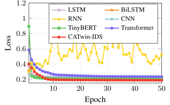
(b) Train loss on CICIDS2018 dataset
