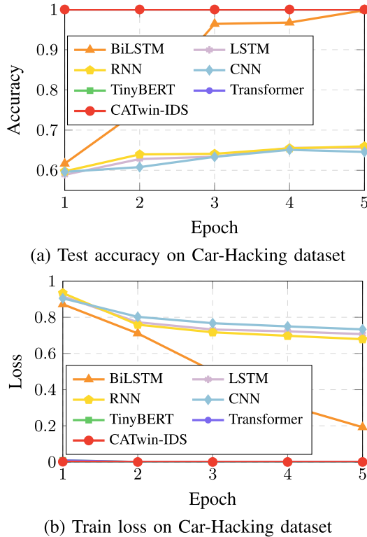
Fig. 7. Comparison of IVN performance indicators on car-hacking dataset.
