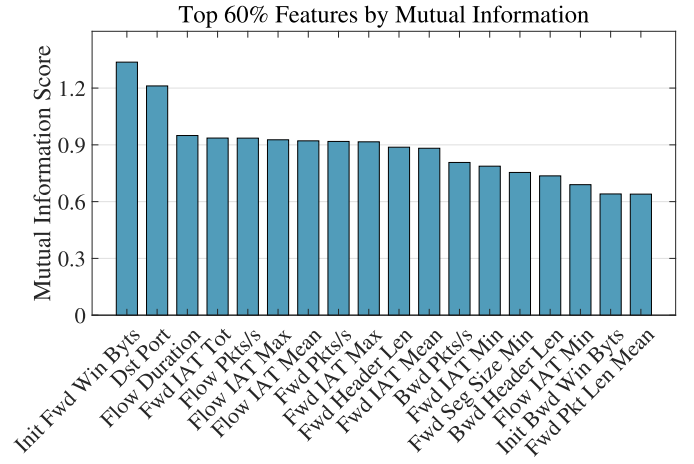
Fig. 4. Selected feature importance from CICIDS2018.
