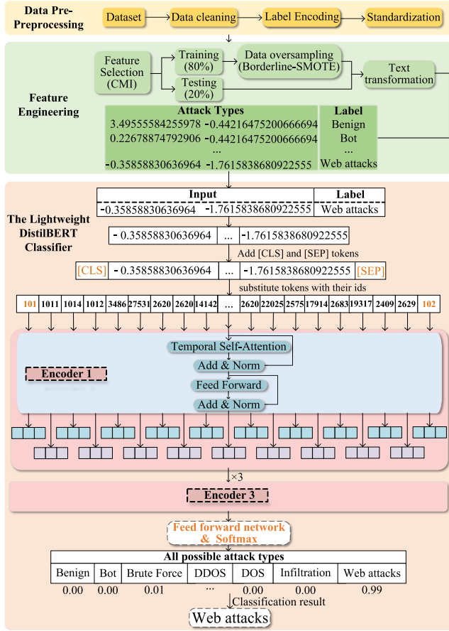
Fig. 3. The overall framework of CATwin-IDS.
