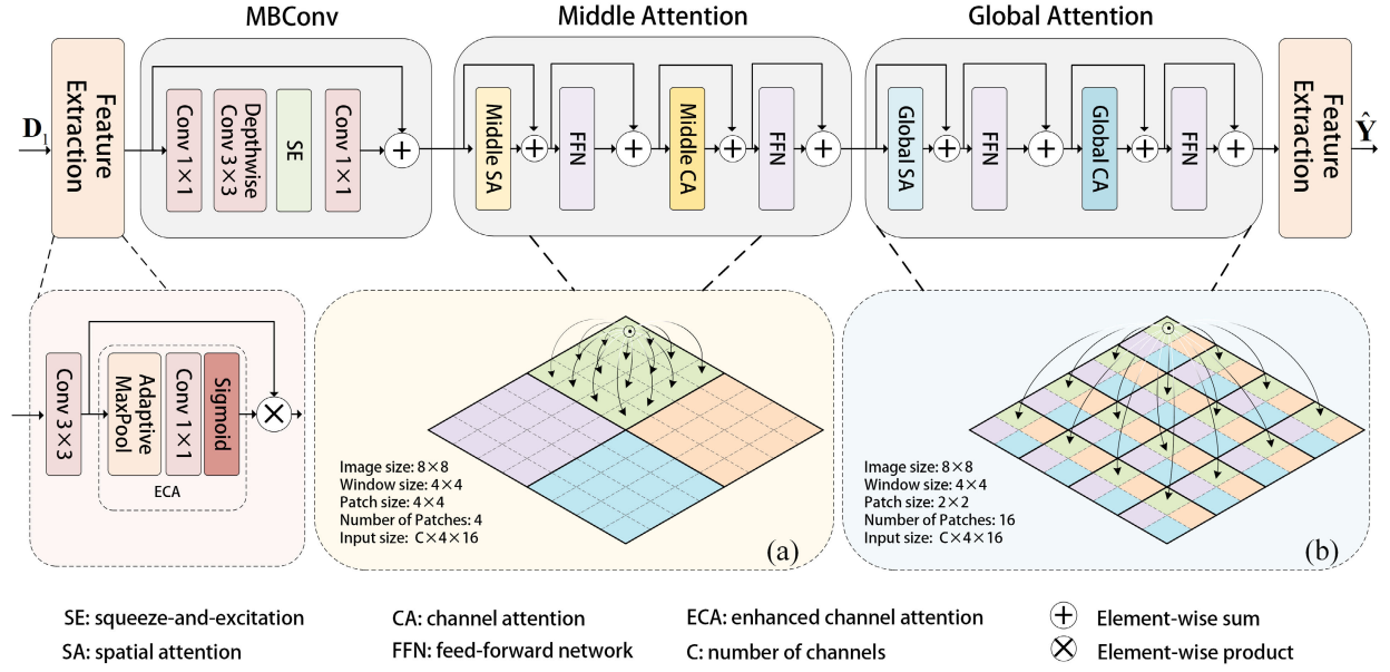
Fig. 5. Background refinement framework with local-middle-global hybrid attention. (a) and (b) Simple examples of generating patches for middle and global attentions, respectively.
