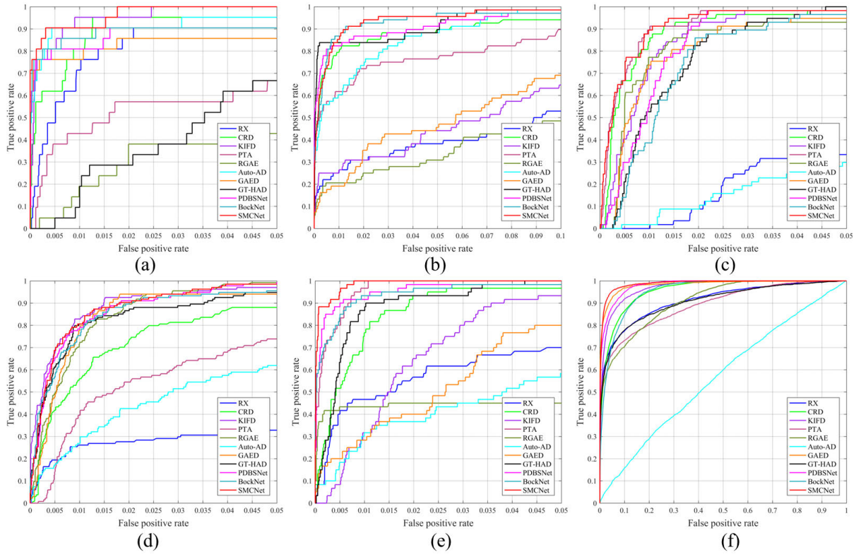
Fig. 11. ROC curves for the considered detectors on six datasets. (a) HYDICE Urban; (b) ABU-B4; (c) San Diego I; (d) San Diego II; (e) Gulfport; and (f) CRi.
