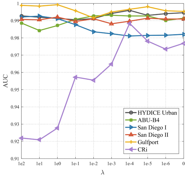
Fig. 7. Sensitivity analysis of SMCNet to parameter \lambda .
