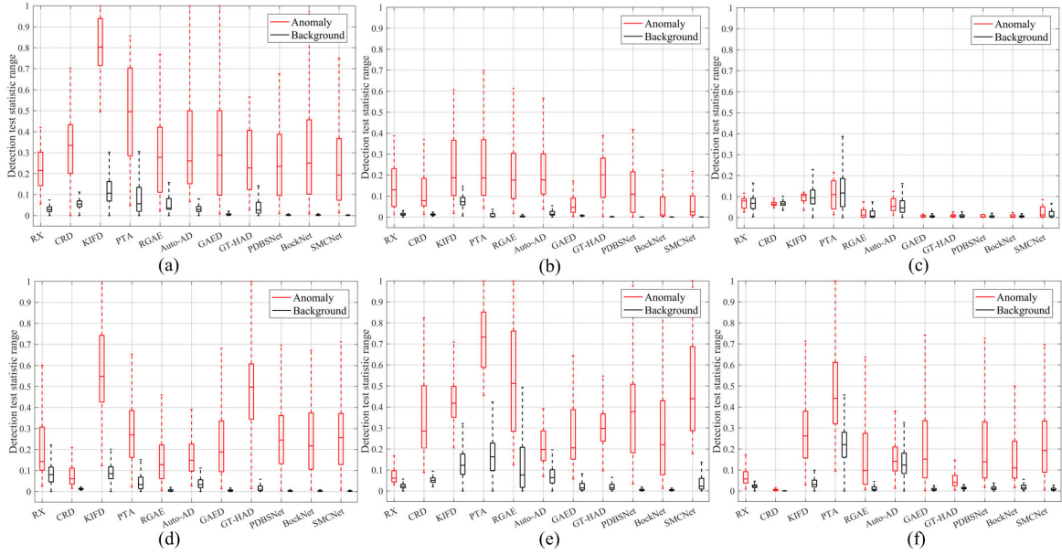
Fig. 10. Box plots of the considered detectors on six datasets: (a) HYDICE Urban; (b) ABU-B4; (c) San Diego I; (d) San Diego II; (e) Gulfport; and (f) CRi.
