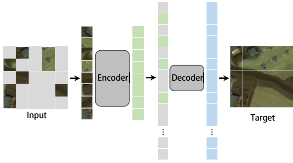
Fig. 1. Graphical illustration of the MAE. The gray patches of the input are the masked regions, which retain the position information. The encoder operates on the visible patches to obtain hidden features, i.e., green patches. Then, the hidden features and the mask tokens (gray patches) are fed into the decoder to reconstruct the image (blue patches).
