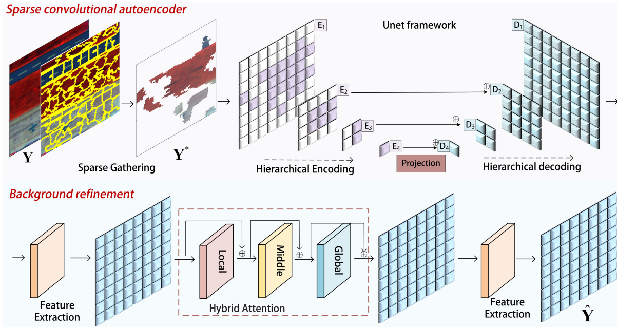
Fig. 2. Architecture of the newly proposed SMCNet, which works to reconstruct the background of the image so that anomalies can be detected by the residual map. First, the input image Y is gathered sparsely using superpixel segmentation and (4)–(6) to retain reliable background information. Then, the masked image Y^* is fed into a Unet framework, as shown in Fig. 4, in which the encoding stage is implemented by employing sparse convolution of the ME library to extract hierarchical features of backgrounds E_1 , E_2 , E_3 , and E_4 . Before decoding, a projection strategy is devised to complement the masked region of the hidden feature map E_4 to generate D_4 . During the decoding stage, D_4 , regular 2-D CNN, and skip connections are used to obtain the decoding feature maps D_1 , D_2 , and D_3 , in which D_1 is the preliminary background reconstruction map with low feature dimensions. After that, a background refinement module composed of two feature extraction layers and a hybrid attention mechanism is deployed, as shown in Fig. 5, to recover the background \hat{Y} completely.
