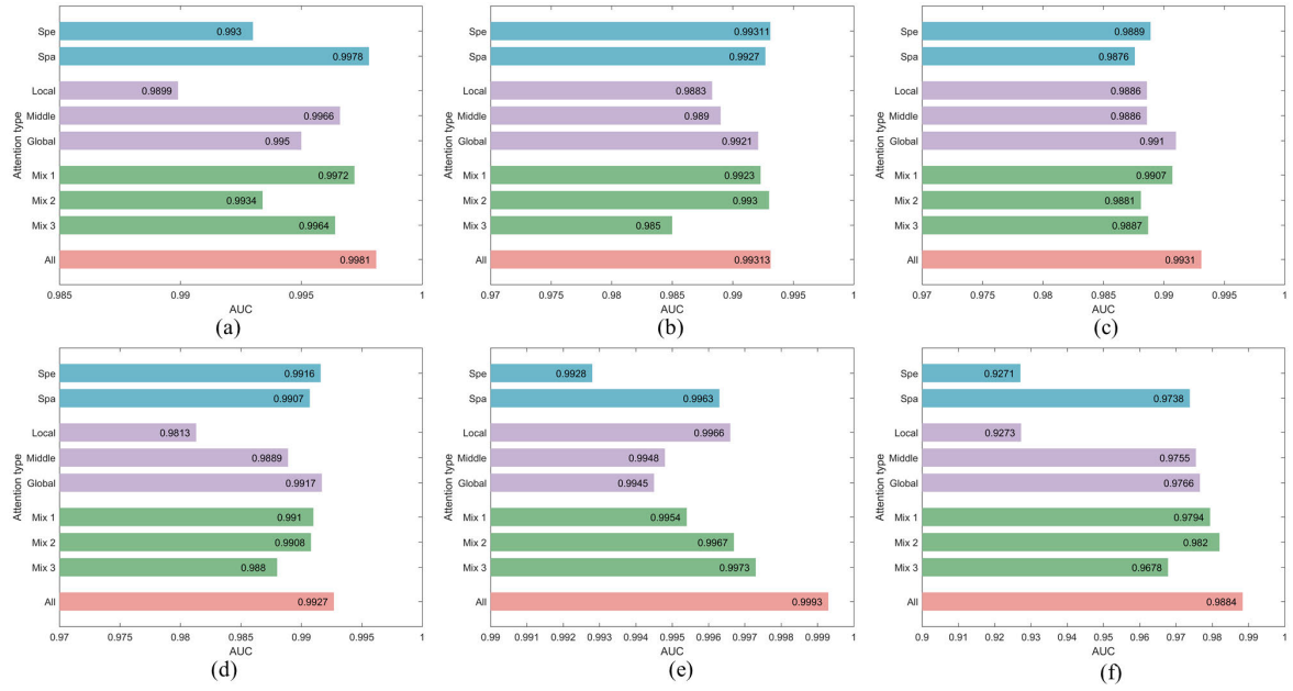
Fig. 8. Comparative results of ablation experiments on hybrid attention for the six considered datasets. (a) HYDICE Urban. (b) ABU-B4. (c) San Diego I. (d) San Diego II. (e) Gulfport. (f) CRI.
