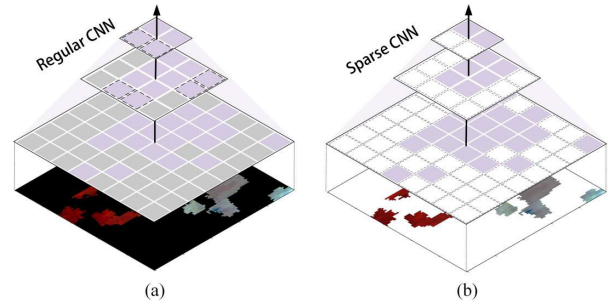
Fig. 3. (a) Regular CNN and (b) sparse CNN for a “holey hyperspectral image” with “empty parts.” The mask regions of the sparse CNN are filled as blank areas, while the mask regions in the regular CNN are filled as gray areas to indicate the zero padding. The regular CNN will change the feature distribution, i.e., the black dashed regions in (a), with the increasing of convolutional layers, while the sparse CNN will keep the original feature distribution.
