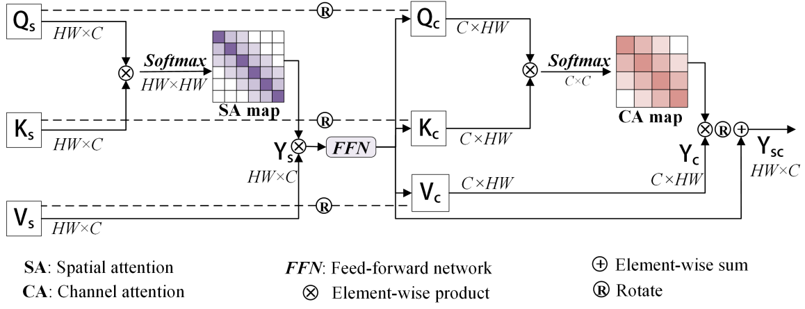
Fig. 6. Graphical illustration of spatial-channel attention.
