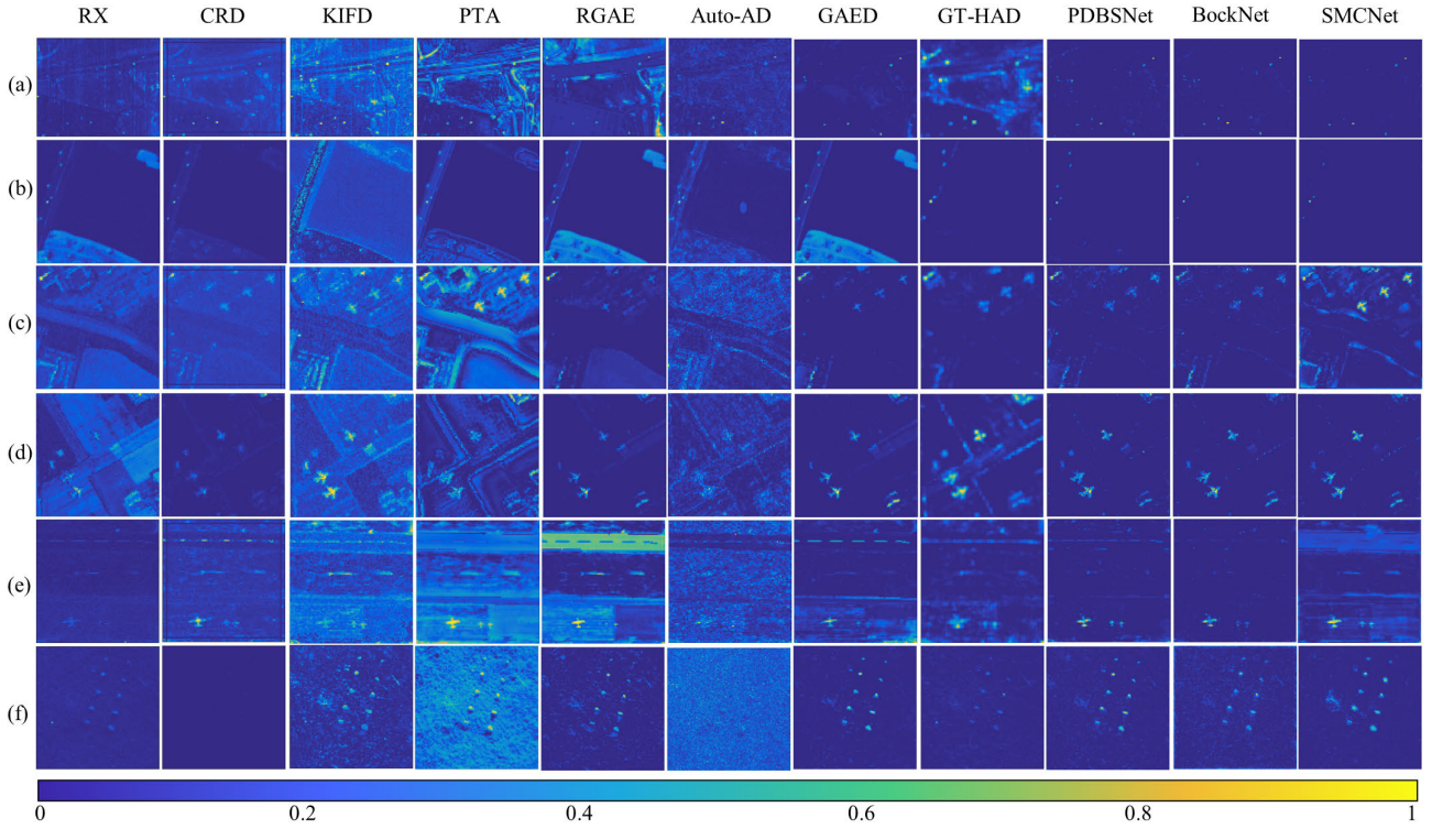
Fig. 9. Anomaly maps produced by the considered detectors on six datasets. From top to bottom: (a) HYDICE Urban; (b) ABU-B4; (c) San Diego I; (d) San Diego II; (e) Gulfport; and (f) CRI.
