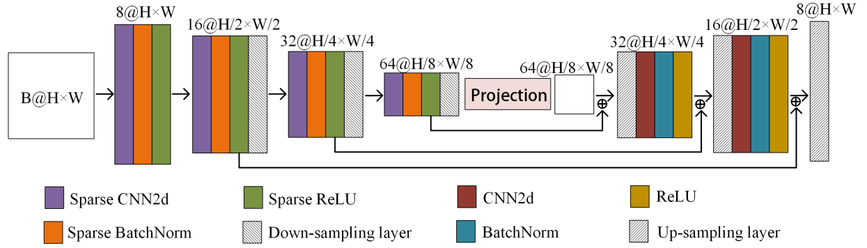
Fig. 4. Structure of the Unet framework by using sparse and regular convolution.
