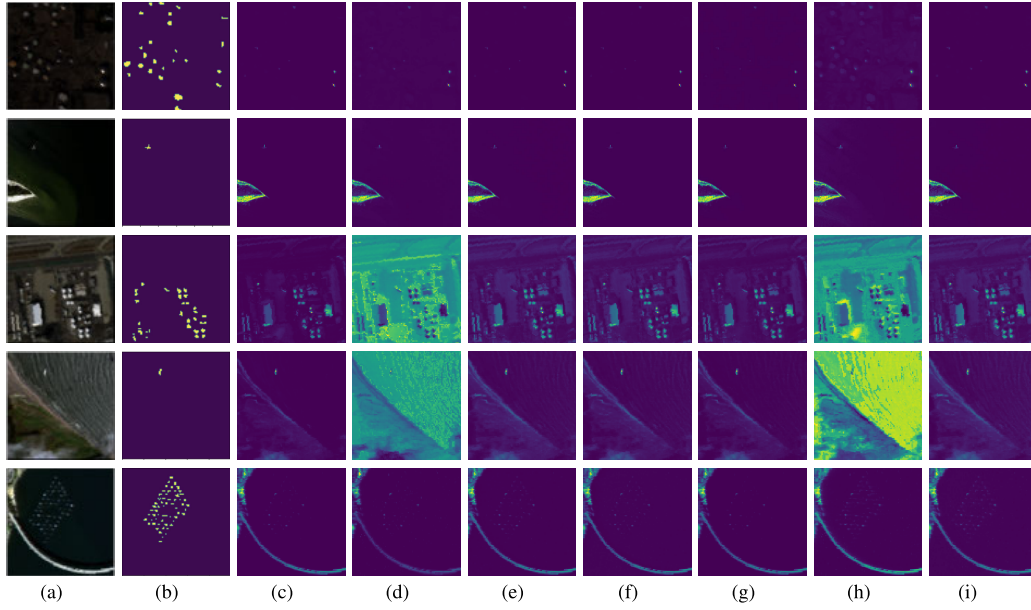
Fig. 7. Visualization for five OHAD results after learning tasks 1–5. The dataset from top to bottom is Los Angeles-1, Cat Island, Los Angeles-2, San Diego, and Bay Champagne, respectively. (a) False color image of HAD. (b) Ground-truth map. (c) J-BioGAN. (d) FT-BioGAN. (e) MAS-BioGAN. (f) EWC-BioGAN. (g) OWM-BioGAN (h) CL-CaGAN. (i) CL-BioGAN.
