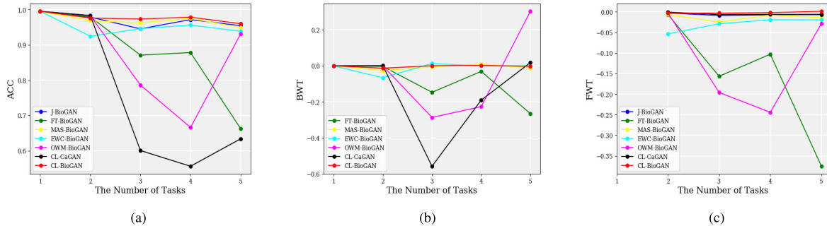
Fig. 5. ACC, BWT, and FWT Performance evaluation for OHAD of different methods. (a) Variation of ACC for tasks 1–5. (b) Variation of BWT for OHAD tasks 1–5. (c) Variation of FWT for OHAD tasks 1–5.
