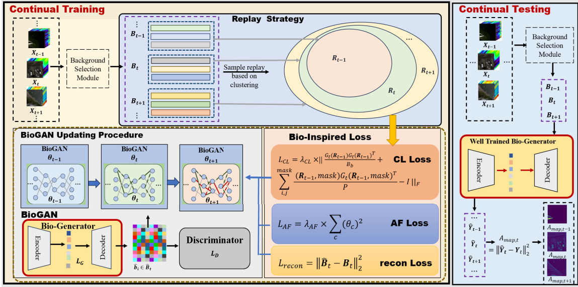
Fig. 3. Overview of the proposed CL-BioGAN for OHAD. The left part represents the continual training phase, which is mainly composed of replay strategy, BioGAN structure, and bioinspired loss (CL Loss, AF Loss, and recon Loss). The right part in the figure is the continual testing part, the well-trained biogenerator is only used in the testing phase to detect the continually arrived HAD scenarios.
