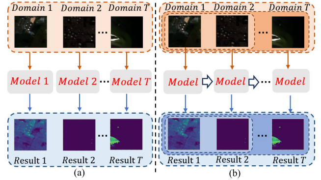
Fig. 1. Comparison of traditional DL training model and the CL method. (a) Traditional DL method, which obtains OHAD results by a set of independent well-trained parameters. (b) Proposed CL method. The parameters of the model are continuously updated with the arrived tasks, but the updated parameters will not forget the previous learned knowledge.
