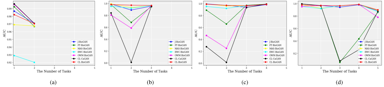
Fig. 4. Catastrophic forgetting performance evaluation for open scenario OHAD on previous tasks. (a) AUC value for tasks 1 and 2 after training on the second task. (b) AUC value for tasks 1–3 after training on the third task. (c) AUC value for tasks 1–4 after training on the fourth task. (d) AUC value for tasks 1–5 after training on the fifth task.
