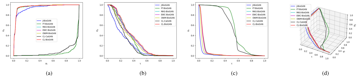
Fig. 6. AUC testing results of different methods on the previous task after learning the fifth task are shown as follows. The first column (a) represents the AUC_{(D,F)} value on Los Angeles-2 after training tasks 1–5. The second column (b) represents the AUC_{(D,T)} value on Los Angeles-2 after training tasks 1–5. The third column (c) represents the AUC_{(F,T)} value on Los Angeles-2 after training tasks 1–5. (d) 3-D ROC value on Los Angeles-2 for tasks 1–5 after completing training on the fifth task.
