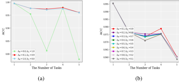
Fig. 8. Varied parameter proportions of \lambda_{AF} and \lambda_{CL} for the detection ACC. (a) Individual impact of \lambda_{AF} and \lambda_{CL} on the experimental results and (b) impact of \lambda_{AF} and \lambda_{CL} on the experimental results within a certain range of values.
