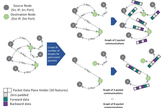
Fig. 2. Graph generation process (only the generation of graph networks for 2 and 3 packets is shown).
