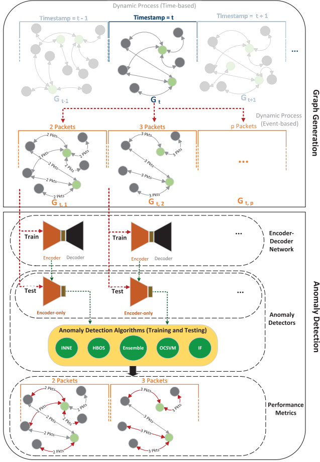
Fig. 1. GTAE-IDS Framework: The anomaly detection process is depicted exclusively for communication graphs involving 2 packets and 3 packets, denoted as G_{t,2} and G_{t,3} , respectively. The red edges displayed at the conclusion of the process within the performance metrics section highlight the anomalous edges identified by the preceding anomaly detection algorithms.
