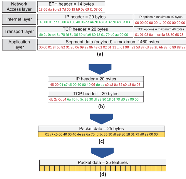
Fig. 3. Packet data structure.
