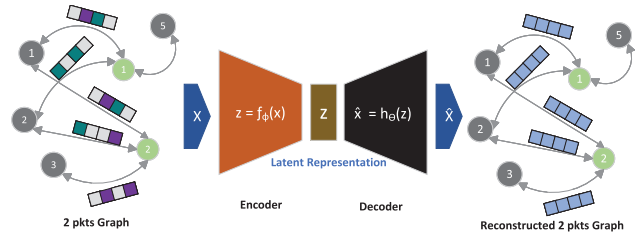
Fig. 5. The graph transformer-based autoencoder model (GTAE).
