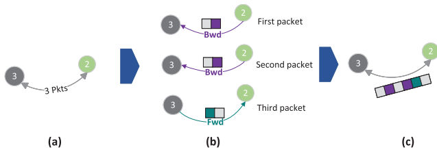
Fig. 4. The edge features encoding process.
