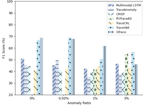
Fig. 17. Algorithm Performance under Different Anomaly Ratios.
