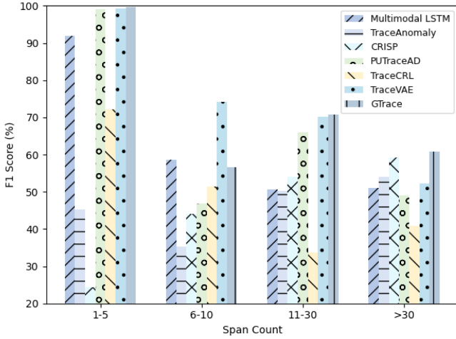
Fig. 15. Algorithm Performance under Different Span Counts.
