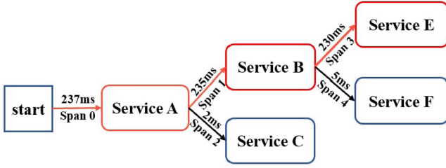
Fig. 2. Latency Anomaly.
