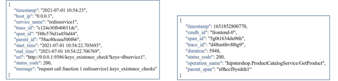
Fig. 8. Different Trace Formats. (a) Data format for GAIA. (b) Data format for AIOps2022.
