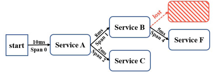
Fig. 4. Structural Anomaly (missing).
