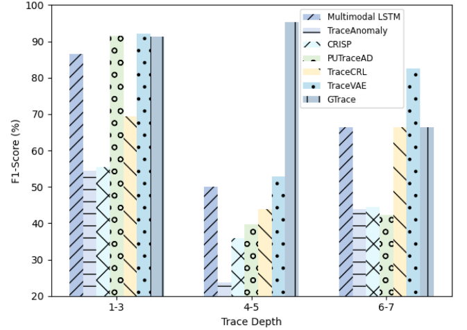
Fig. 14. Algorithm Performance under Different Trace Depths.
