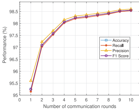
Fig. 1. Performance of FDL model in binary scenario based on X-IIoTID dataset.
