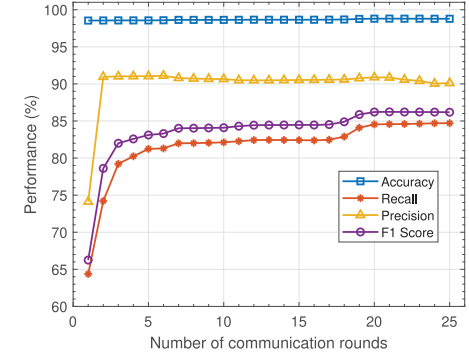
Fig. 5. Performance of FDL model in 6-class scenario based on Edge-IIoTset dataset.
