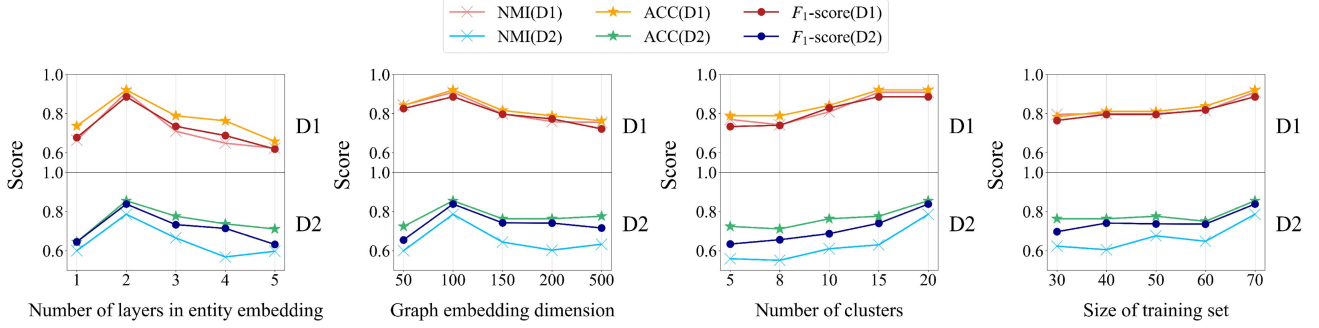
Fig. 4. Hyperparameters sensitivity on UniDiag .
