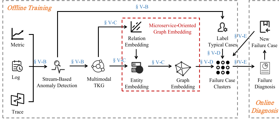
Fig. 2. The framework of UniDiag .
