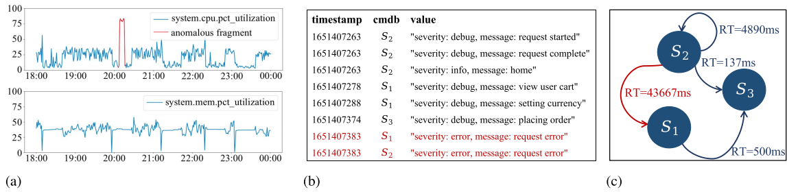
Fig. 1. An example of the multimodal data of a microservice system during a failure. Fig. 1(a) shows two metrics; the blue line in the figure represents the original value of the metric, and the red line represents an anomalous fragment. Fig. 1(b) shows eight logs; the red ones are anomalous. Fig. 1(c) shows a trace where a node represents a microservice instance, an edge from a caller to a callee denotes a span, and the red span is anomalous because of its excessively high response time.
