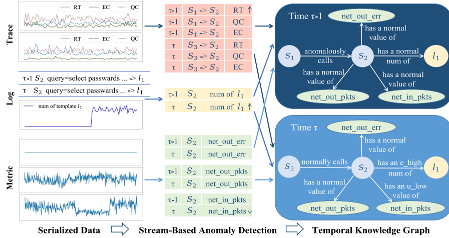
Fig. 3. Multimodal data serialization, stream-based anomaly detection, and construction of TKGs (u_low: unexpectedly low, e_high: excessively high).
