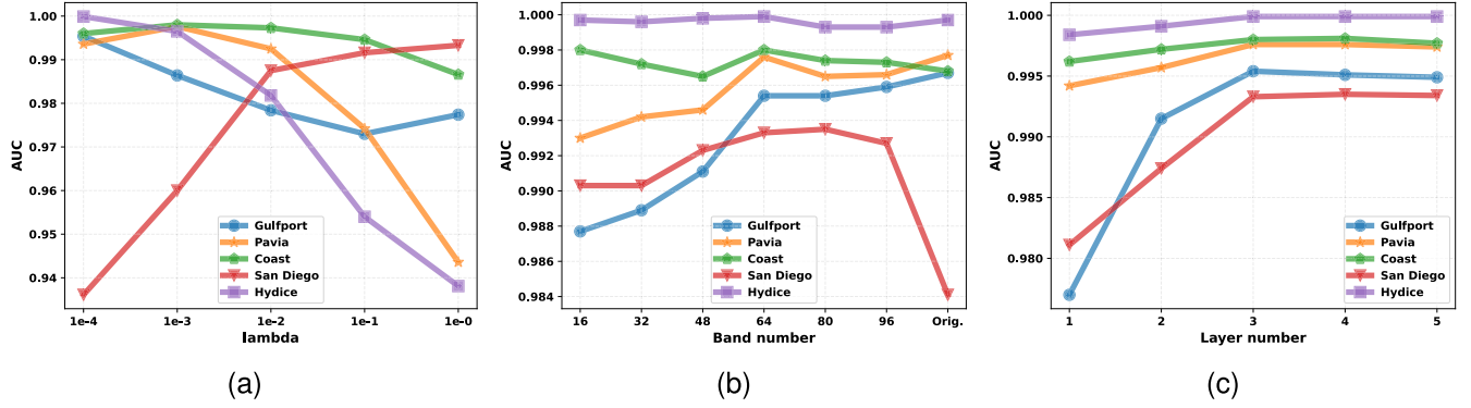
Fig. 10. Analysis of hyperparameters using AUC of (P_d, P_f) as metric on the classic datasets. (a) Regularization parameter \lambda . (b) Band number N_{bs} . (c) Layer number L . Datasets Gulfport, Pavia, Coast, San Diego, and Hydice are, respectively, shown as blue, orange, green, red, and purple curves.
