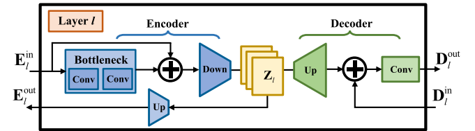
Fig. 3. l -th CED layer. The input feature \mathbf{E}_l^{\text{in}} of layer l first undergoes a bottleneck module and residual skip processing, followed by a down block to obtain \mathbf{Z}_l . Subsequently, \mathbf{Z}_l splits into two branches: the first one passes through the up block in the encoder part, producing \mathbf{E}_l^{\text{out}} for lower layers; the second one goes through the up block in the decoder part, and after fusing with the decoder features \mathbf{D}_l^{\text{in}} from lower layers, it yields the output feature \mathbf{D}_l^{\text{out}} for layer l .
