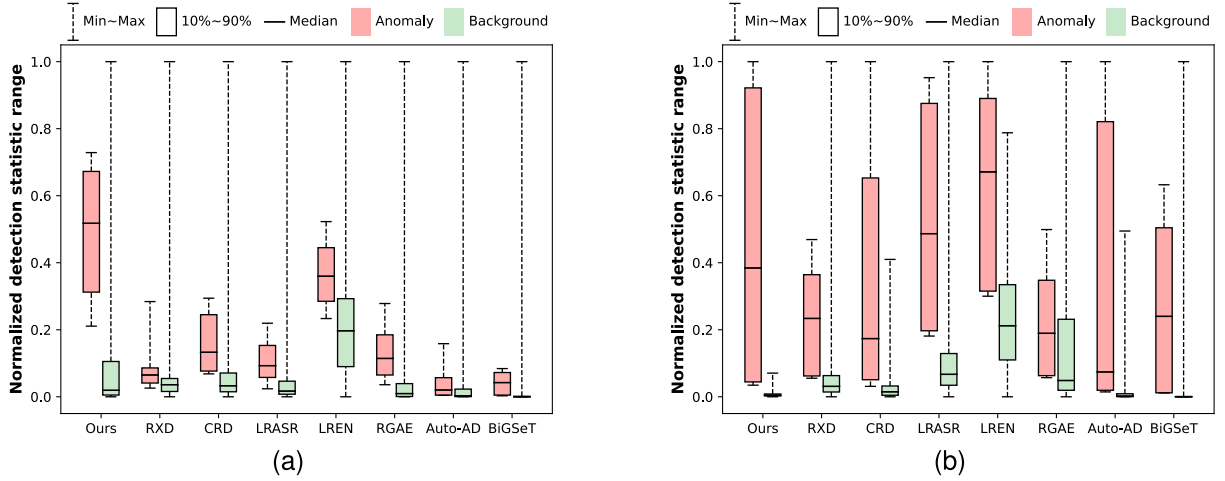
Fig. 9. Background-anomaly separability results for different methods on (a) San Diego and (b) Hydice datasets.
