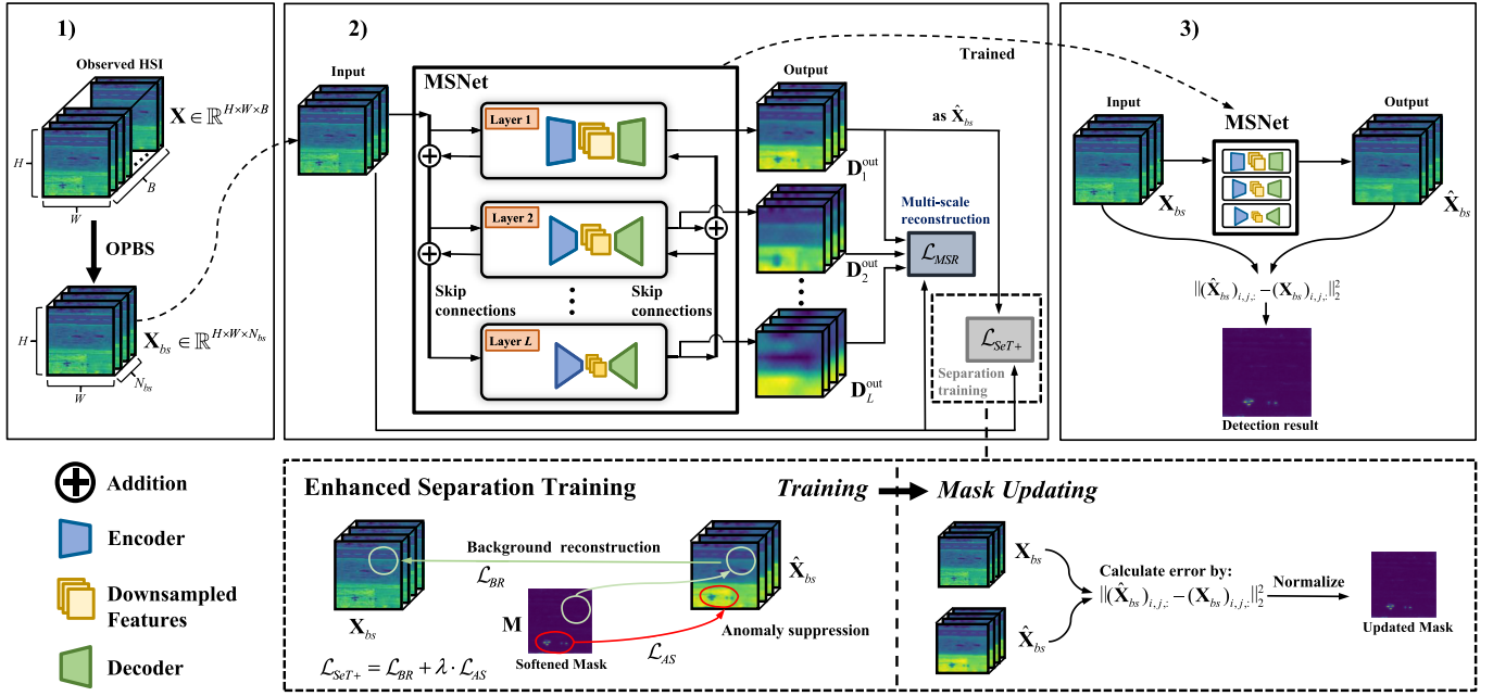
Fig. 2. Overview of our proposed MSNet method. Our detection consists of three steps. 1) Band selection, 2) multiscale network training, and 3) network inference to obtain the detection result. We use OPBS before training to remove band redundancy from the input HSI while preserving its discriminability. The MSNet architecture consists of L stacked multiscale layers, each of which serves as a downscaling feature learner at a different scale. Skip connections in summation trunks are employed to fuse both encoding and decoding features. We train the network using two losses including the multiscale reconstruction loss \mathcal{L}_{MSR} and the enhanced separation training loss \mathcal{L}_{SeT+} . The output decoded features \mathbf{D}^{\text{out}} are regarded as different scale levels of \mathbf{X}_{bs} constrained by \mathcal{L}_{MSR} as the content to retain both deep and shallow multiscale characteristics in the network. The topmost feature \mathbf{D}_1^{\text{out}} is designated as the reconstructed background and undergoes separation training with \mathbf{X}_{bs} . In enhanced separation training, we use an adaptively updated soft latent mask to separately represent background and anomaly regions, reconstructing the background part while suppressing the anomaly part without the need for threshold fine-tuning. The final detection result is obtained by computing the error between the input image and the background computed from network inference.
