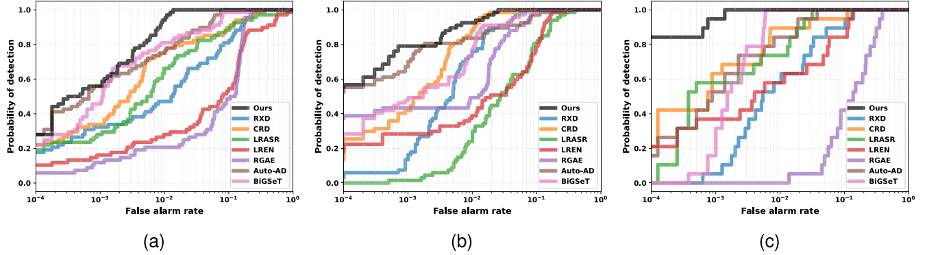
Fig. 7. ROC curves of (P_d, P_f) for different methods on (a) Pavia, (b) Coast, and (c) Hydice datasets.
