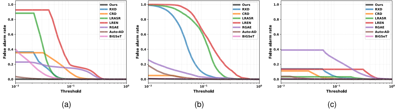
Fig. 8. ROC curves of (P_f, \tau) for different methods on (a) Pavia, (b) Coast, and (c) Hydice datasets.
