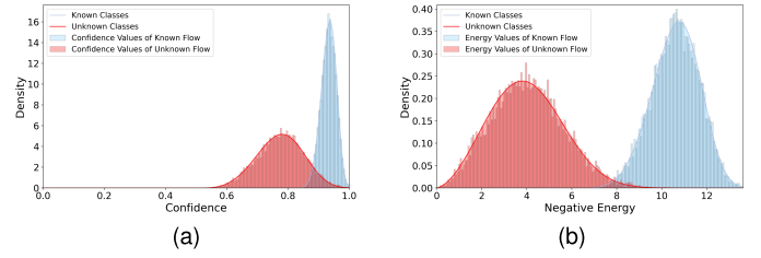
Fig. 11. Comparison between the distributions of (a) Softmax confidence scores and (b) energy values from the EBM.
