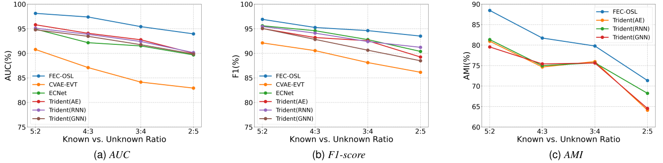
Fig. 5. Evaluation of the AUC, F1 score, and AMI metrics under different known/unknown class ratios on the CIC-IDS-2018 dataset.
