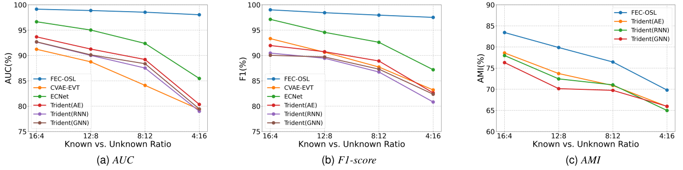
Fig. 4. Evaluation of the AUC, F1 score, and AMI metrics under different known/unknown class ratios on the USTC-TFC-2016 dataset.
