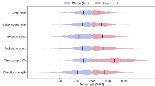
Fig. 9. Feature importance for Weibo and Zeus flows. The violins depict the per-sample |shape| distributions of each interaction feature. The vertical bars indicate the median SHAP values, reflecting the central contribution of each feature for Weibo (left, blue) and Zeus (right, red) flows.
