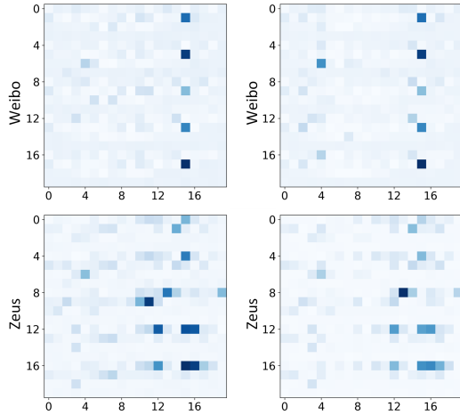
Fig. 8. Header-byte attention heatmaps for Weibo and Zeus flows. Darker colors indicate higher model attention to the corresponding byte regions during inference.
