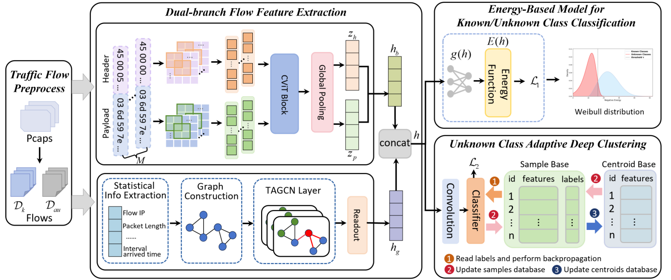
Fig. 2. Overall structure of FEC-OSL. The model is trained in an end-to-end manner using a combination of cross-entropy loss, energy-based regularization loss and clustering loss.
