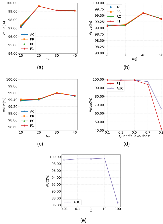
Fig. 12. Impact of various hyperparameters on FEC-OSL performance.
