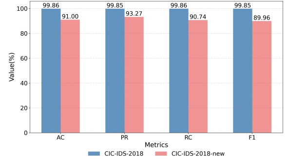
Fig. 10. Results of concept drift evaluation.
