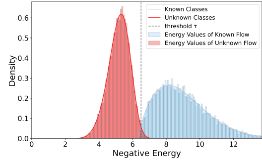
Fig. 3. Comparison of the negative energy Weibull distributions for known and unknown flows. The histogram shows the density distributions of known classes (blue) and unknown classes (red) across different energy ranges. The dashed line indicates the threshold used to distinguish between known and unknown classes.
