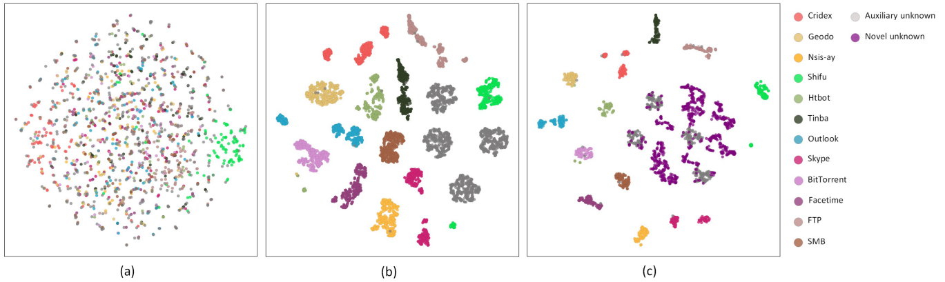
Fig. 7. Visualization of feature space at different stages. (a) Before training: known (colored) and auxiliary unknown (grey) flows are mixed. (b) After training: known flows form compact clusters, and unknown flows are well separated. (c) Testing: novel unknown flows (purple) remain clearly separated from known clusters.
