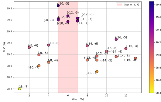
Fig. 13. Impact of energy-boundary parameter combinations ( m_k, m_u ) on open-set recognition performance. The x-axis represents the absolute margin |m_u - m_k| , while the y-axis shows the AUC values for each parameter pair. The color of each point represents the corresponding performance, with darker shades indicating a higher AUC.
