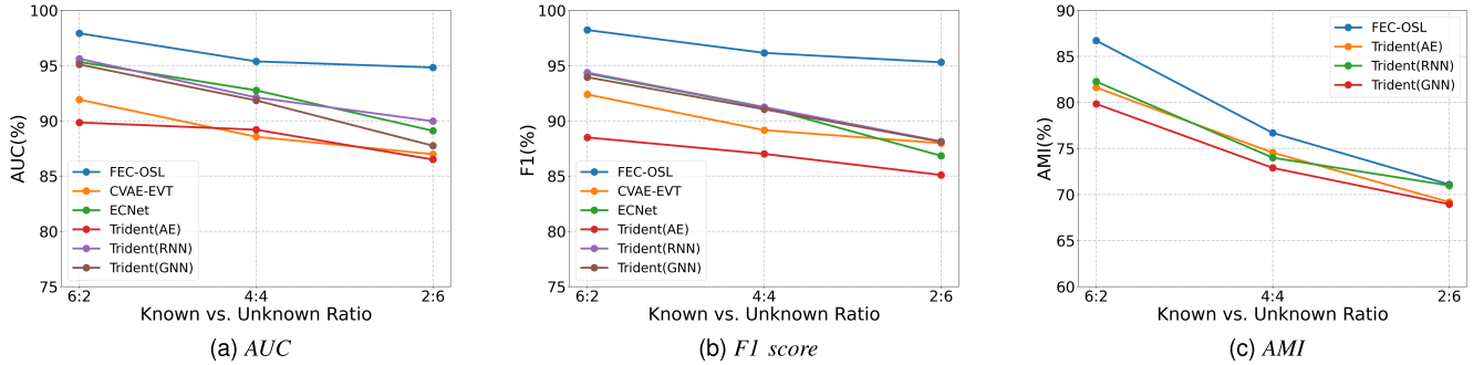
Fig. 6. Evaluation of the AUC, F1 score, and AMI metrics under different known/unknown class ratios on the ISCX-Tor-2016 dataset.
