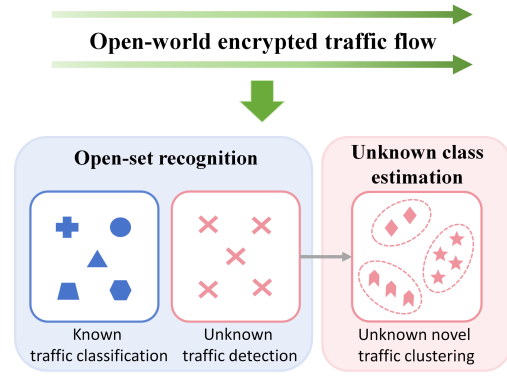
Fig. 1. Schematic of an open-world fine-grained classification task for known and unknown encrypted traffic, including the distinction between known and unknown traffic, classification of known classes, and clustering of unknown classes.
