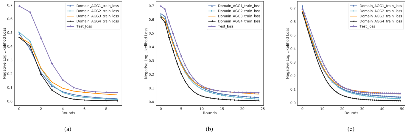
Fig. 3. Learning curves for (a) 10 rounds; (b) 25 rounds; and (c) 50 rounds.
