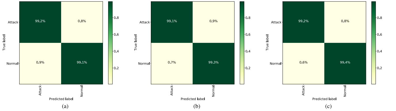
Fig. 4. Confusion matrices for Binary classification for (a) 10 rounds; (b) 25 rounds; and (c) 50 rounds.
