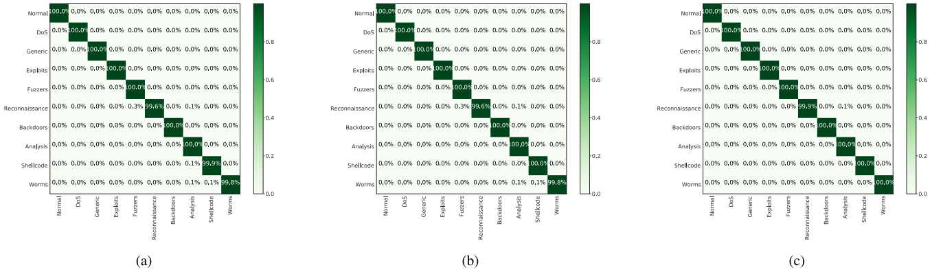
Fig. 5. Confusion matrices for Multi-class Classification for (a) 10 rounds; (b) 25 rounds; and (c) 50 rounds.
