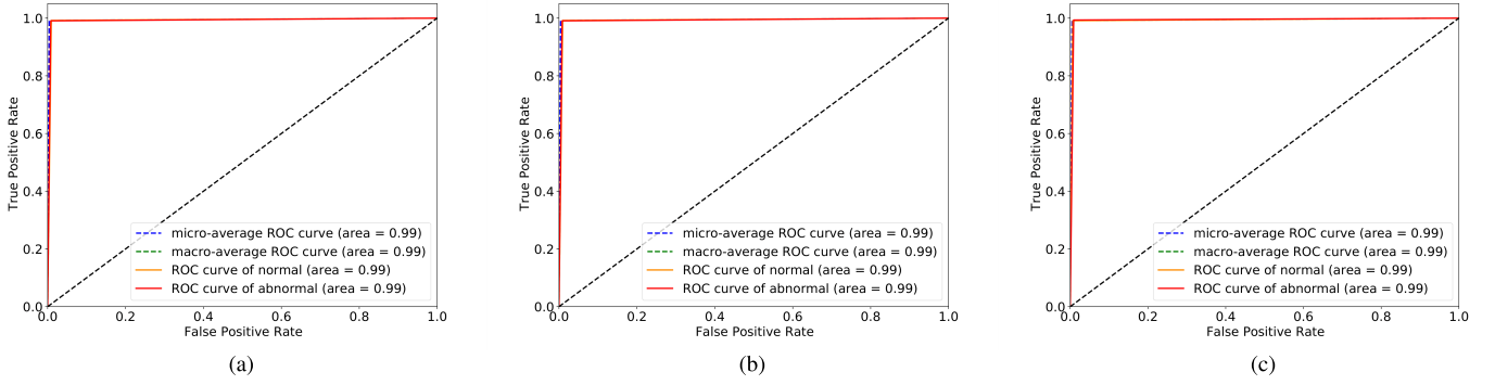
Fig. 6. ROC Curves for Binary classification for (a) 10 rounds; (b) 25 rounds; and (c) 50 rounds.
